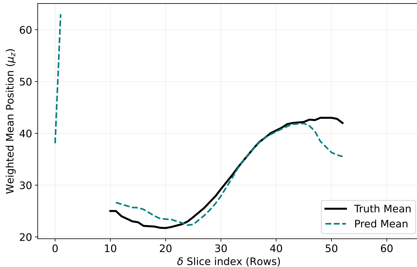
Mean Profile of Constant- \delta Slices
