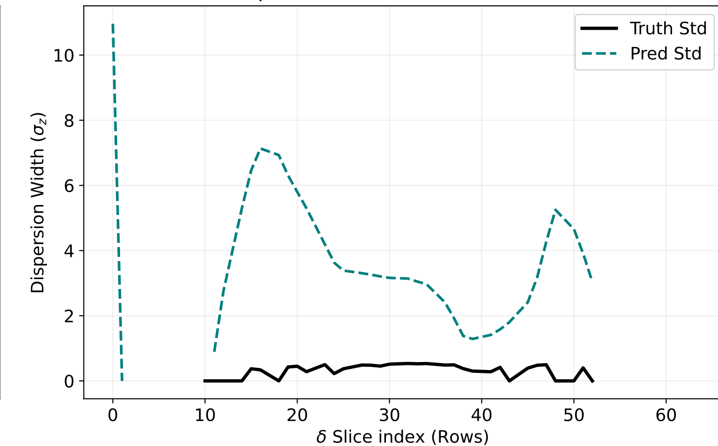
Dispersion ( \sigma ) of Constant- \delta Slices
