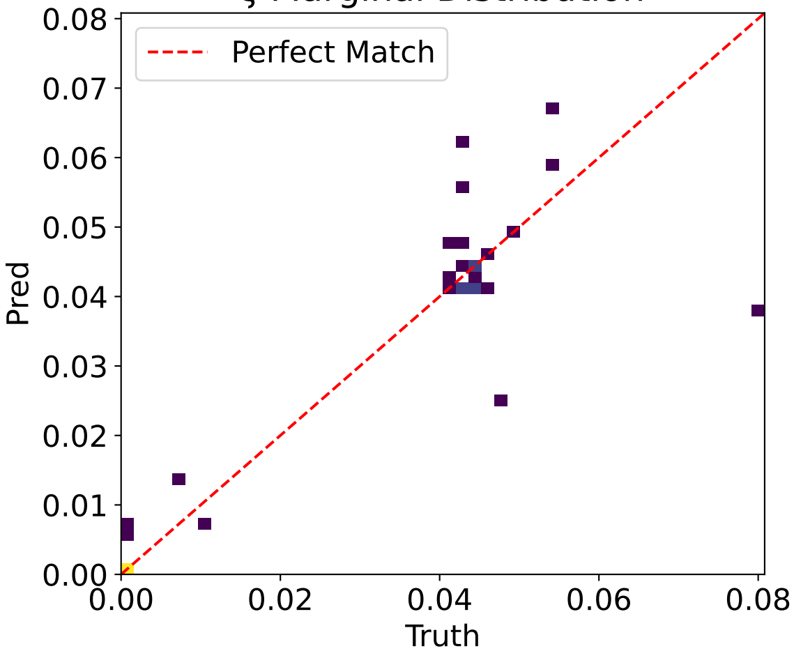
\zeta Marginal Distribution
