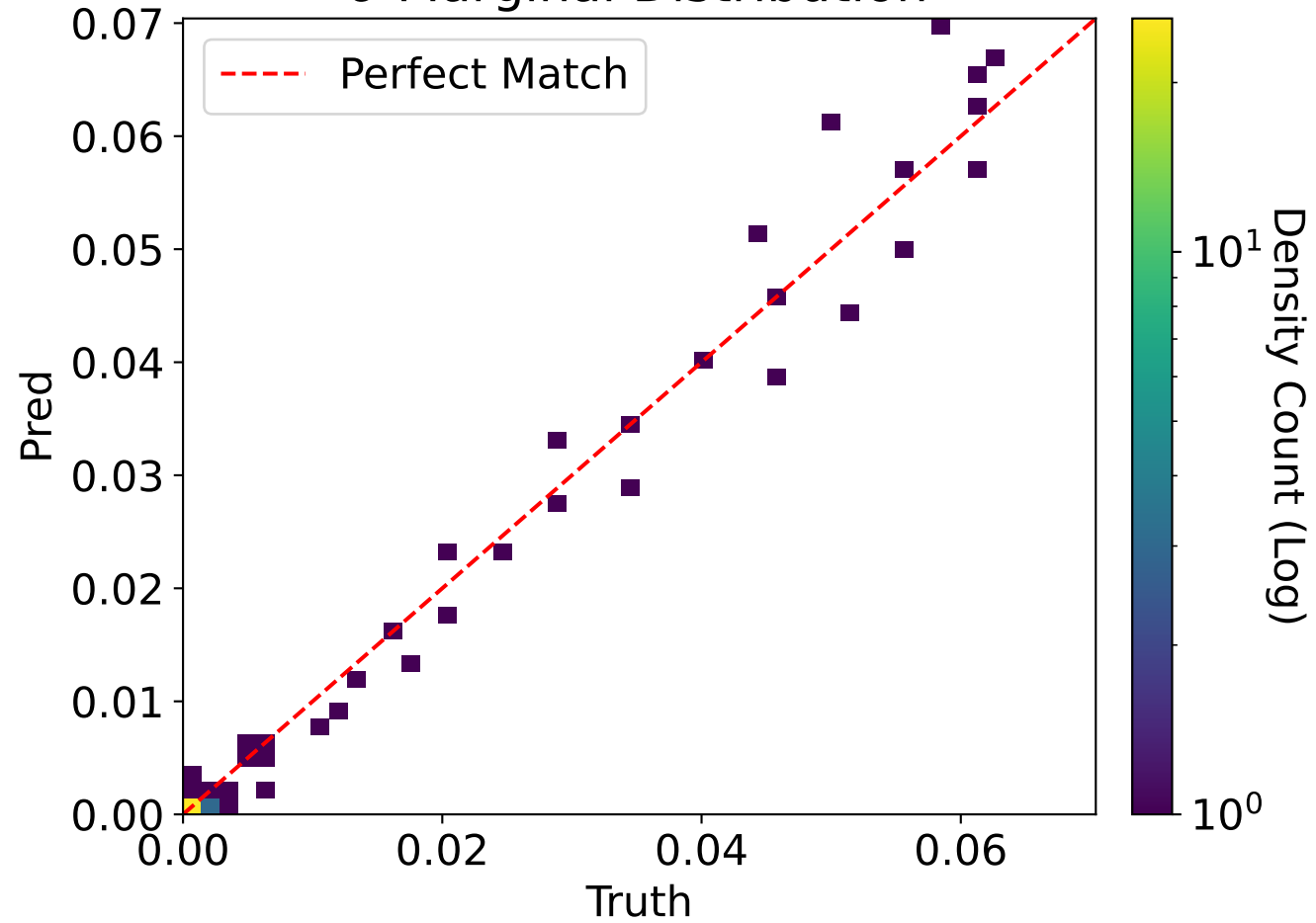
\delta Marginal Distribution
