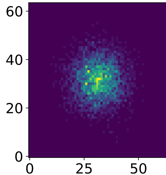
Ground Truth
