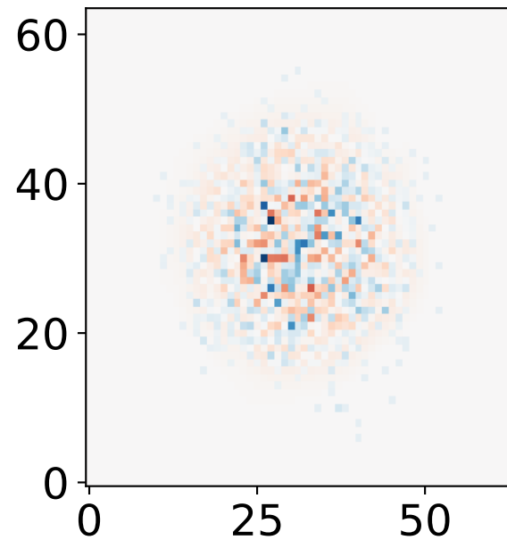
Transformer Error
