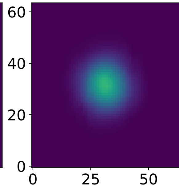
Transformer Pred
