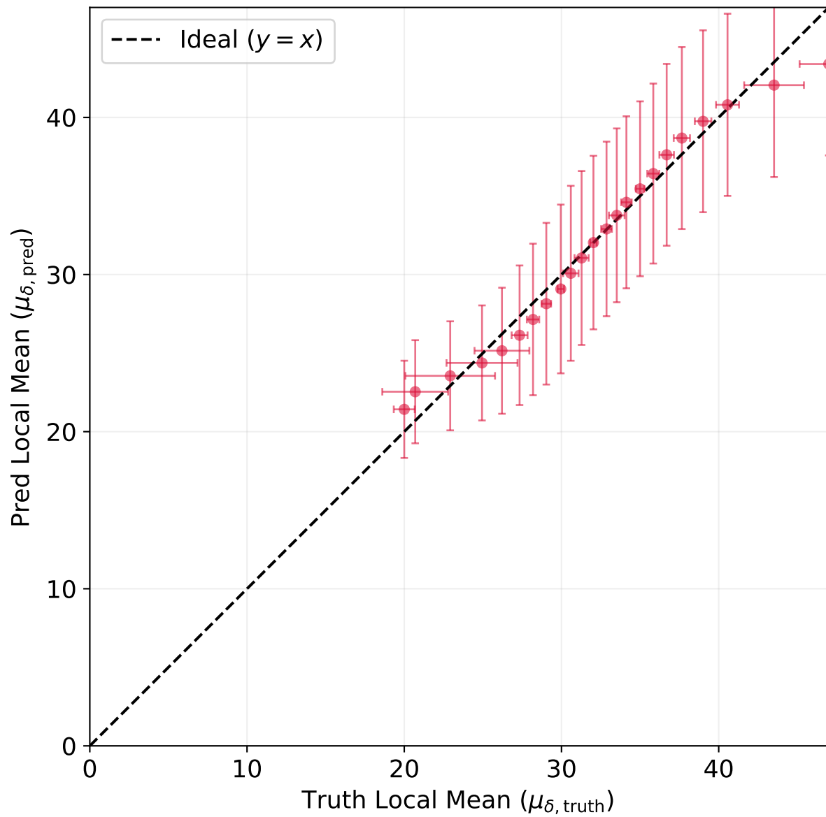
Constant-z Slices ( \delta Distribution Means)
