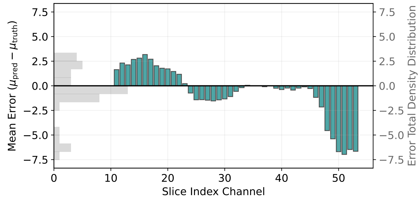
z Mean Residuals vs Slice Index
