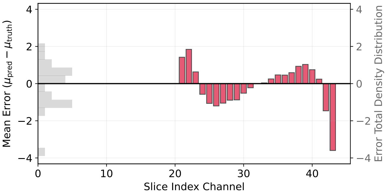
\delta Mean Residuals vs Slice Index
