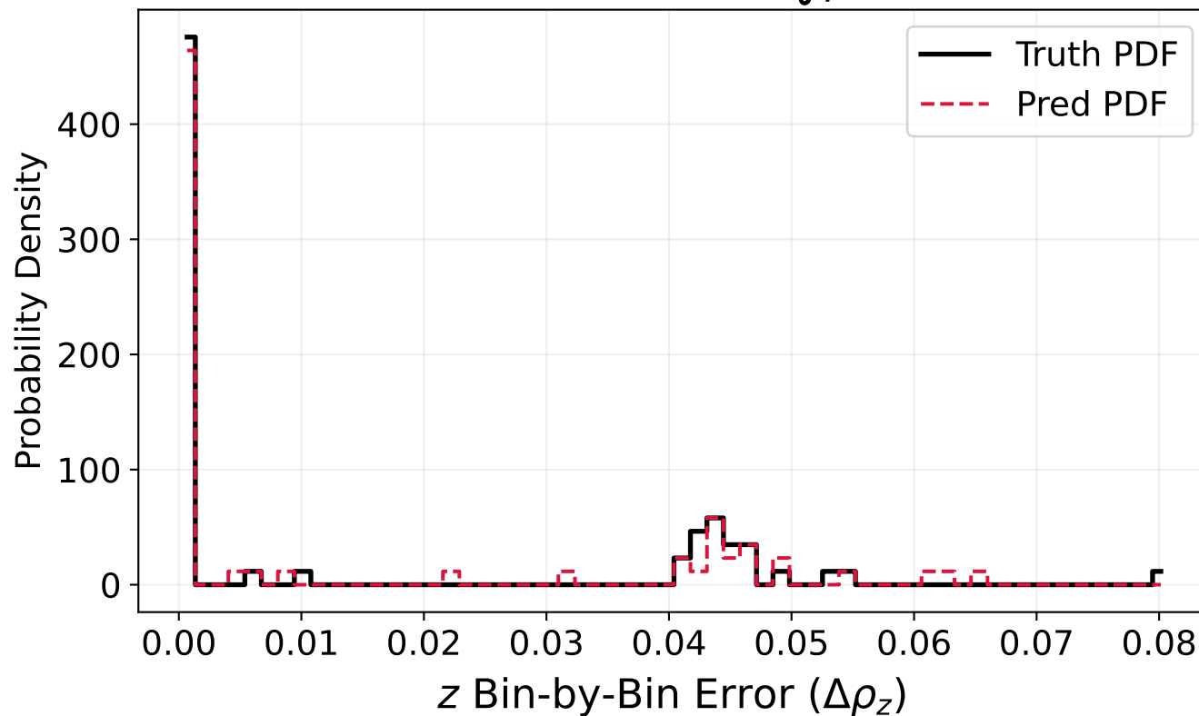
z Normalized PDFs ( \int \rho_z = 1 ) Normalized Probability Density Diagnostics Normalized PDFs ( \int \rho_\delta = 1 )
