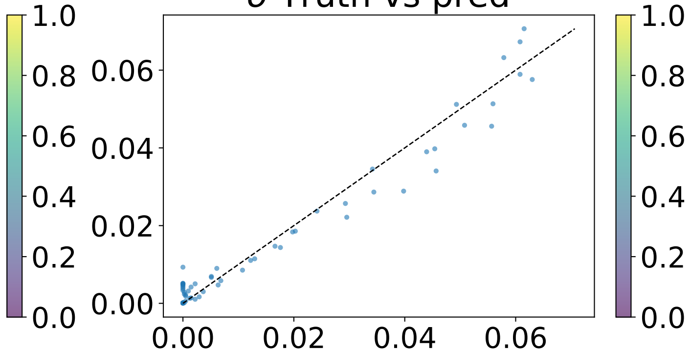
sample 3 pair ( z, \delta )
