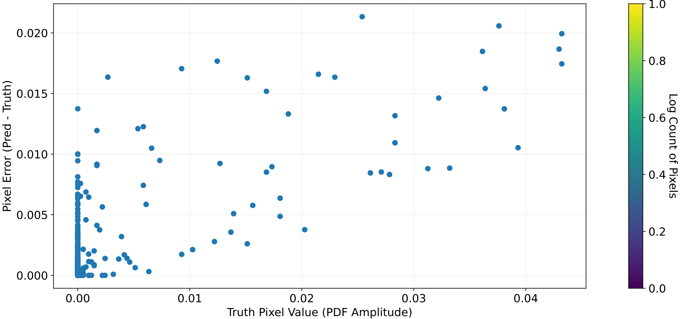
Pixel-by-Pixel PDF Error Space ( z, \delta )
