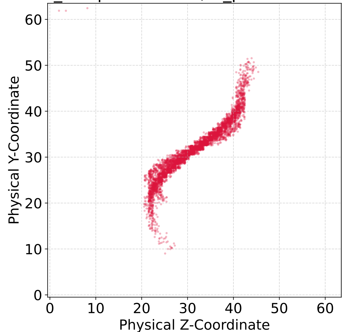
Sampled Macroparticles (Scatter) N_sampled=50000, N_plotted=5000
