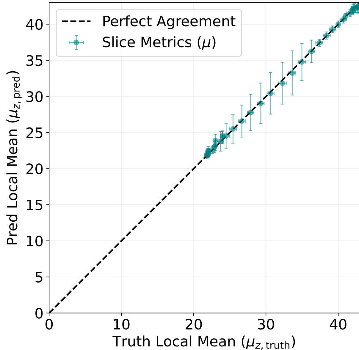
Constant- \delta Slices ( z Distribution Means)
