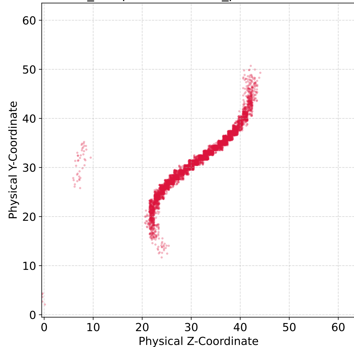
Sampled Macroparticles (Scatter) N_sampled=50000, N_plotted=5000
