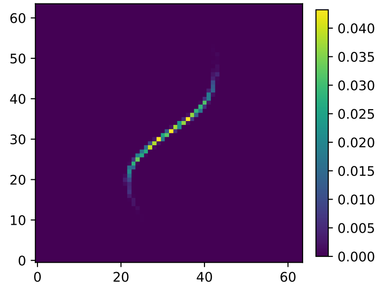
Truth
