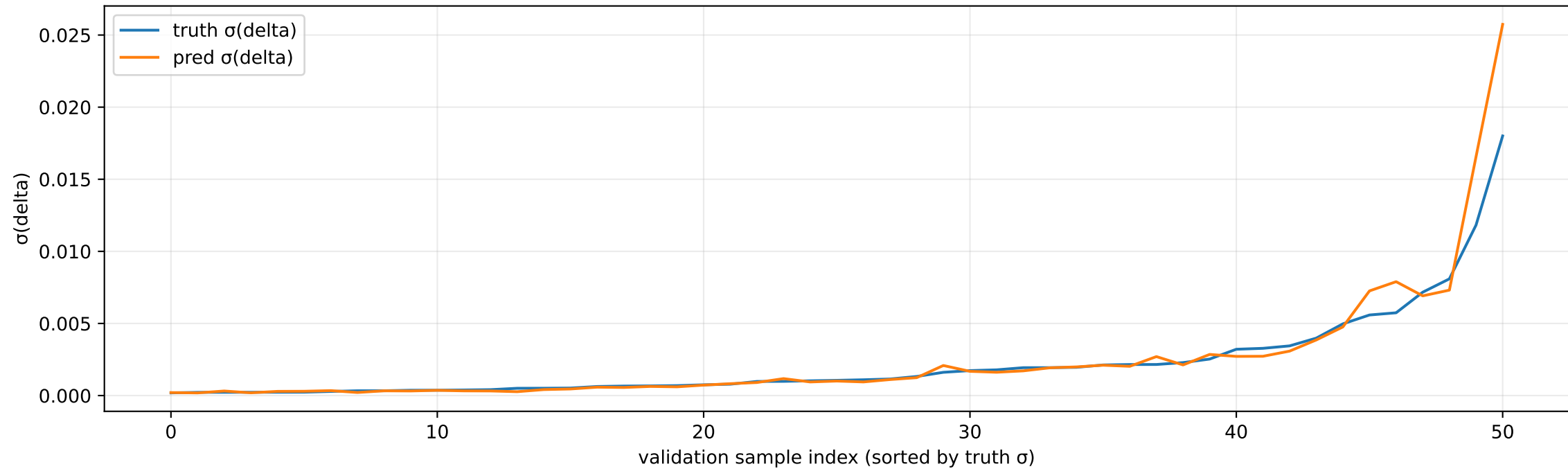
\sigma(\text{delta}) vs index: prediction vs truth
