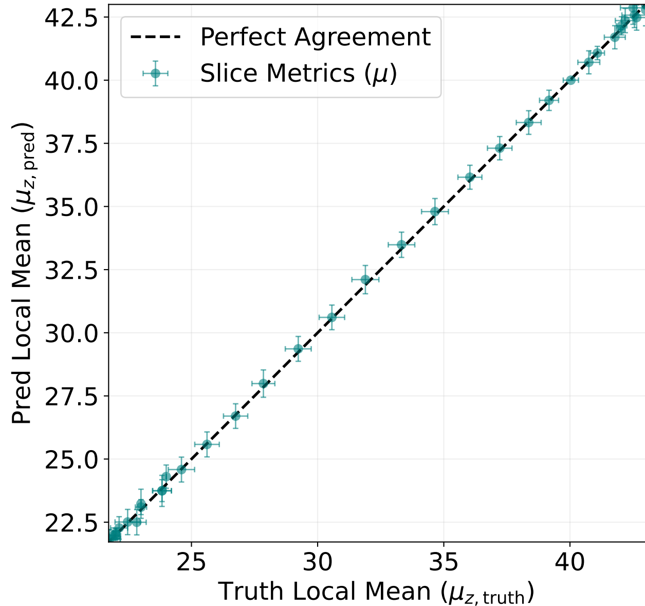
Constant- \delta Slices ( z Distribution Means)
