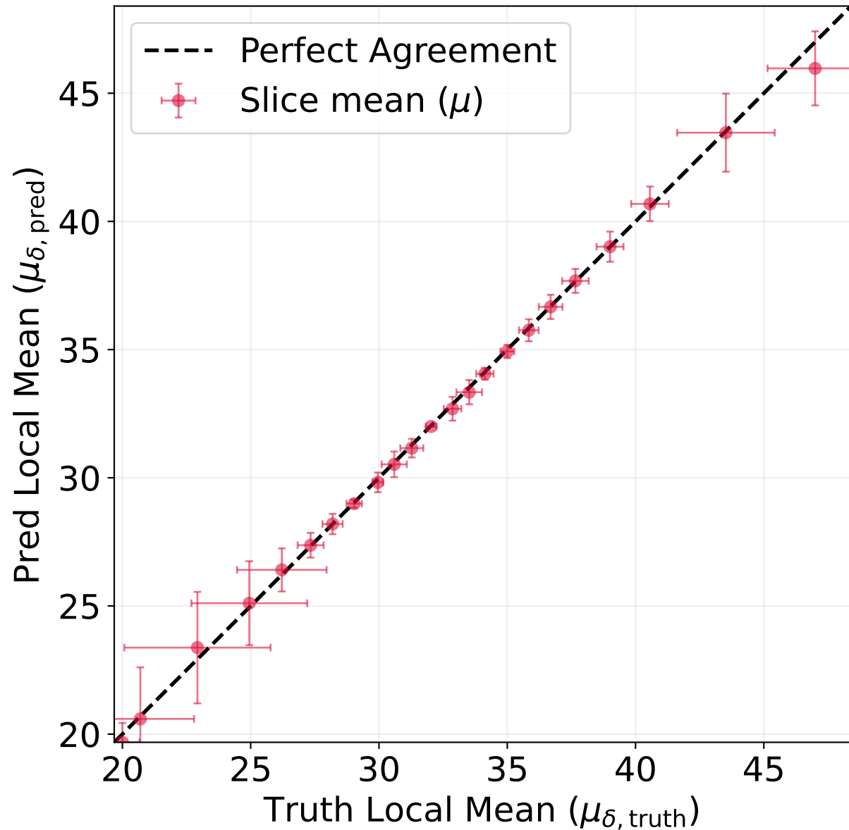
Constant- z Slices ( \delta Distribution Means)
