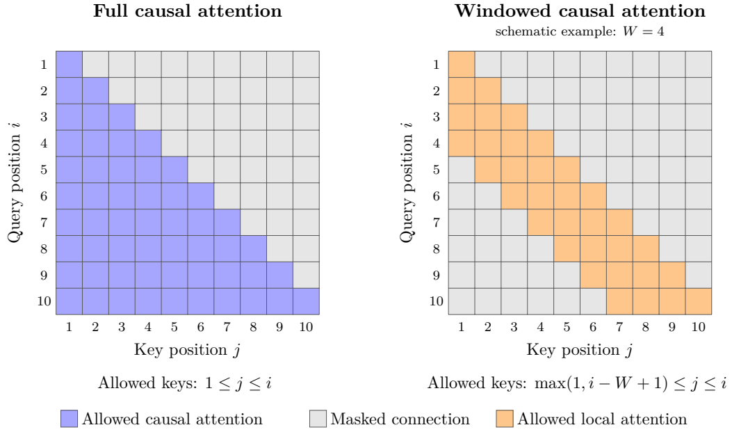
Fig. 5: Comparison of the attention support used by the full causal and windowed Transformer variants. Rows correspond to query positions i and columns to key positions j .
