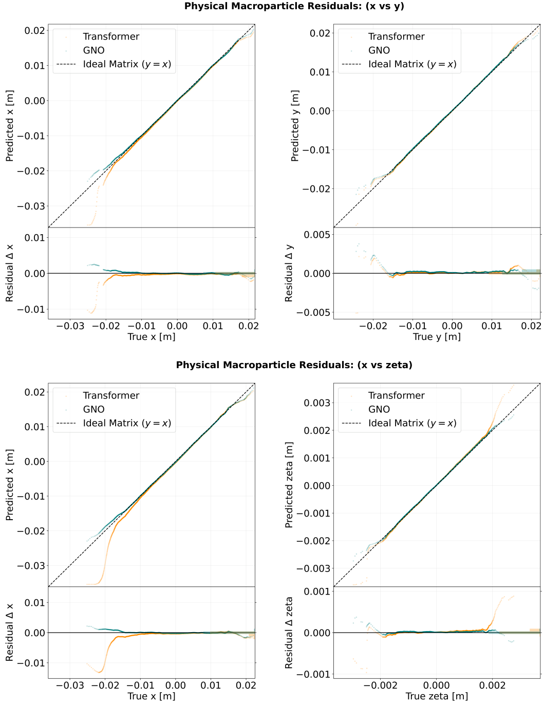
Fig. 15: Macroparticle-based comparison for sample s = 3 . Top: (x, y) projection. Bottom: (x, \zeta) projection. Synthetic particles are sampled from the reference, local-window Transformer, and GNO density maps. Parity and residual diagnostics reveal distributional displacement in physical coordinates.
