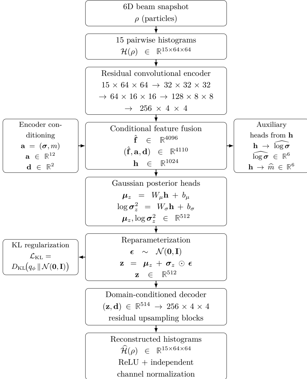
Fig. 4: Implemented conditional variational autoencoder architecture used to construct the reduced representation of six-dimensional beam snapshots.
