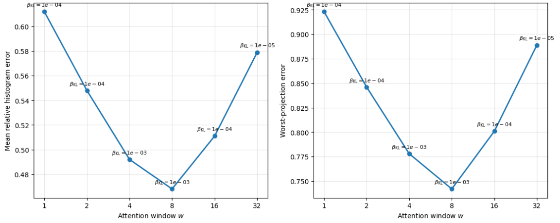
Fig. 16: Transformer window-size study after independent selection of the KL regularization weight \beta_{KL} for each causal attention window w . The left panel reports the mean relative histogram error across the reconstructed phase-space projections, while the right panel shows the corresponding worst-projection error. The results exhibit an intermediate optimum: very narrow attention provides insufficient context, whereas increasingly broad windows progressively degrade the reconstruction after the minimum reached near w = 8 .
