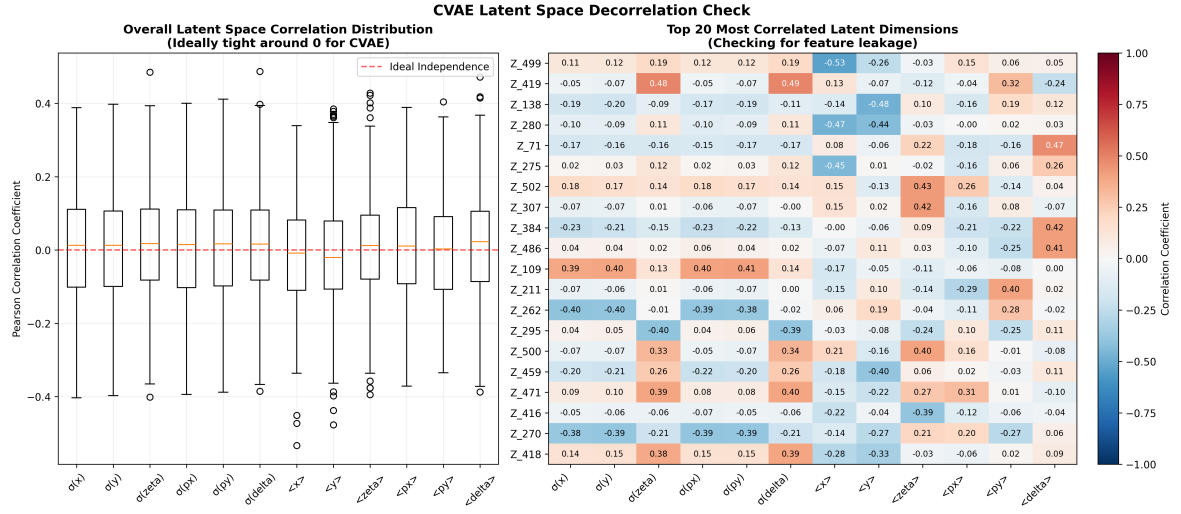
Fig. 10: Pearson-correlation diagnostics between the CVAE latent representation and the auxiliary physical beam statistics. The left panel shows the distribution of signed correlation coefficients across the 512 latent coordinates for each of the 12 physical observables, comprising the six coordinate-wise rms spreads \sigma = (\sigma_x, \sigma_y, \sigma_\zeta, \sigma_{p_x}, \sigma_{p_y}, \sigma_\delta) and the six phase-space centroids \langle \mathbf{x} \rangle = (\langle x \rangle, \langle y \rangle, \langle \zeta \rangle, \langle p_x \rangle, \langle p_y \rangle, \langle \delta \rangle) . The right panel displays the full correlation patterns of the 20 latent coordinates attaining the largest absolute correlation with any physical observable. The signed distributions remain concentrated around zero and no single physical statistic produces a systematic displacement of the latent population.
