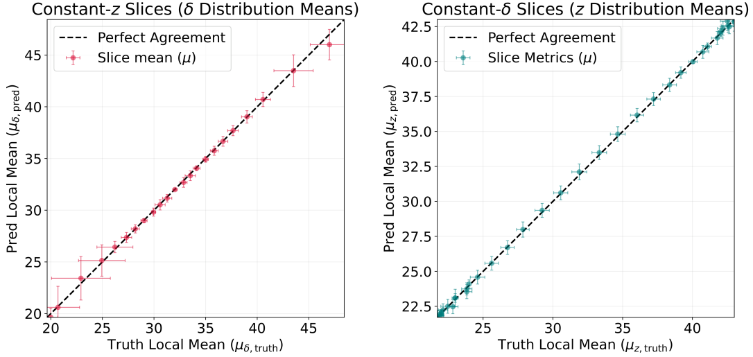
Fig. 11: Conditional-slice consistency of the local-window Transformer for the longitudinal (\zeta, \delta) marginal. The diagnostic compares predicted and reference conditional means for constant- \zeta and constant- \delta slices. Error bars encode local conditional spread. Concentration around the ideal parity relation indicates preservation of internal longitudinal phase-space structure beyond agreement of global moments.
