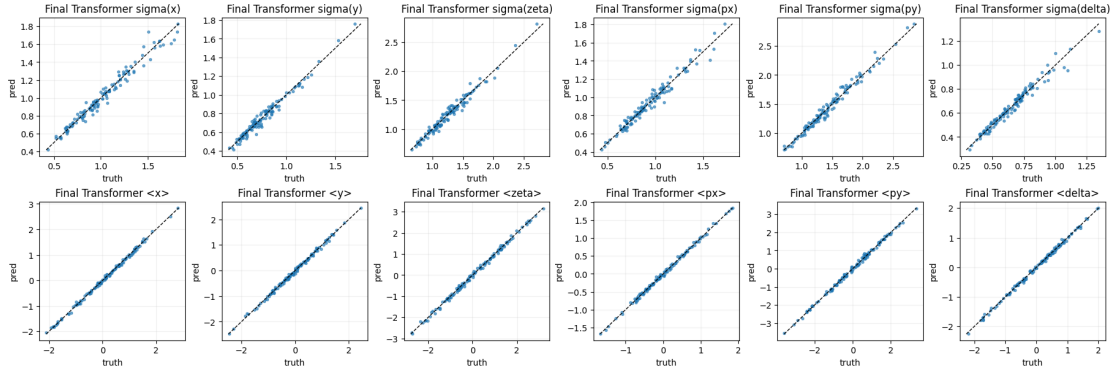
Fig. 17: Parity comparison for the physics-statistics prediction head. Predicted beam centroids and RMS spread extensions are compared with their reference values across the six phase-space coordinates. Agreement with the diagonal indicates accurate reconstruction of the corresponding first- and second-order beam statistics, while deviations from the y = x line quantify systematic bias and prediction error.
