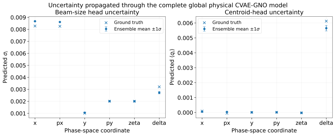
Fig. 20: Conditional latent variability of the six predicted coordinate-wise RMS spreads and six centroids for validation sample s = 3 . Circles and error bars show the ensemble mean and one posterior-sampling standard deviation over R = 100 stochastic forward passes, crosses show the corresponding reference values. Raw coordinate units are shown in the figure, while the dimensionless physical errors are summarized in Table 12. The intervals quantify sensitivity to conditional latent sampling only and are not calibrated confidence intervals.
