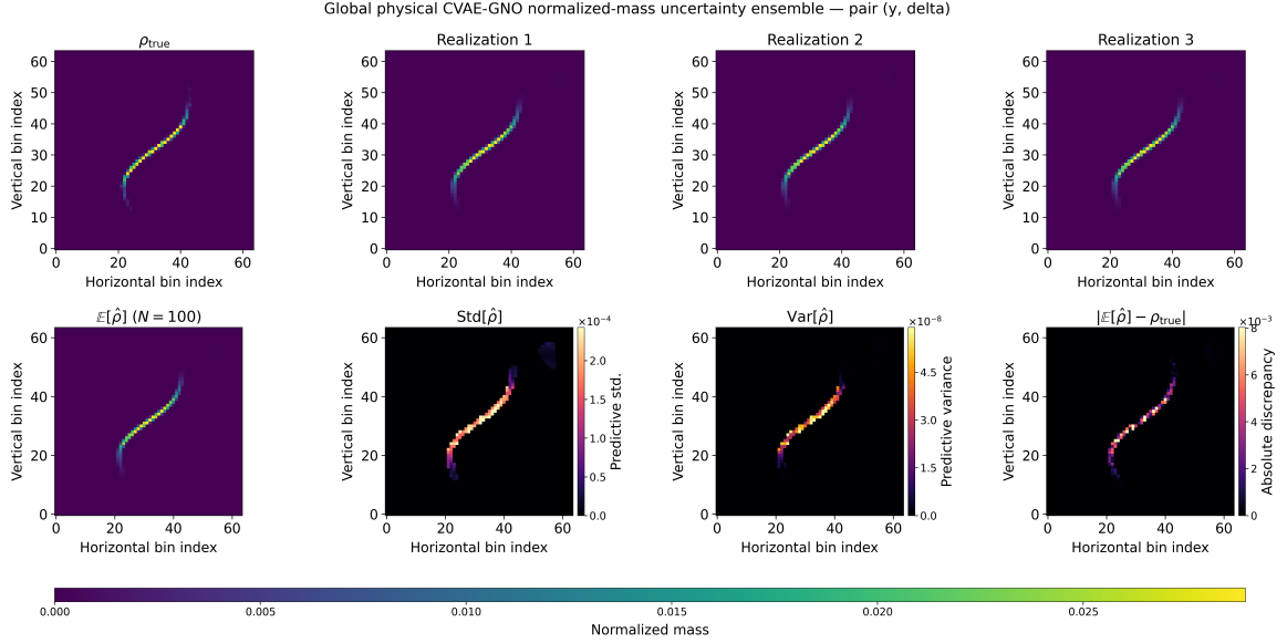
Fig. 18: Conditional latent uncertainty for the normalized (y, \delta) histogram mass of validation sample s = 3 , obtained from R = 100 stochastic CVAE samples propagated through the complete GNO surrogate. The panels compare the reference distribution, representative posterior draws, the ensemble mean, predictive standard deviation, predictive variance, and absolute ensemble-mean discrepancy. Because the histogram is normalized, this figure isolates variability of the decoded distributional shape before physical rescaling.
