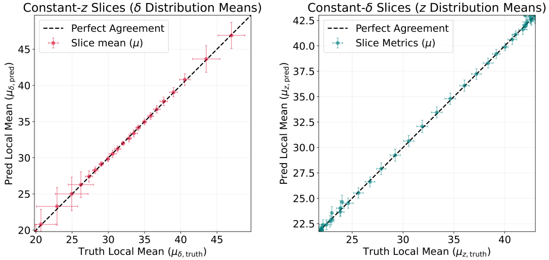
Fig. 12: Conditional-slice consistency of the CVAE-GNO surrogate for the longitudinal (\zeta, \delta) marginal. The figure evaluates agreement of local conditional means under constant- \zeta and constant- \delta slicing. Comparison with Fig. 11 isolates differences in internal phase-space reconstruction between local-window attention and graph-kernel propagation.
