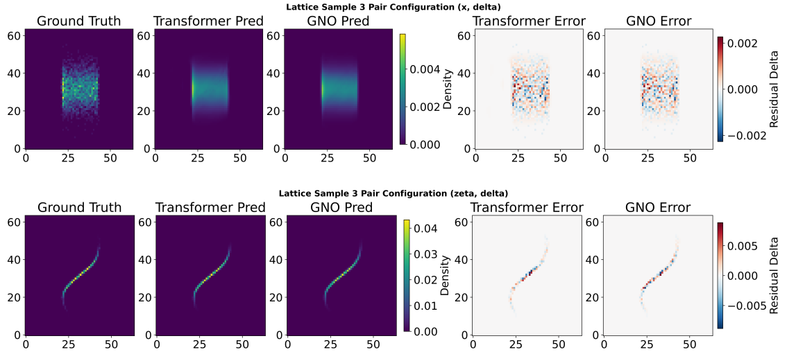
Fig. 14: Direct density-level comparison of the local-window Transformer and GNO for sample s = 3 . Top: mixed transverse–energy marginal (x, \delta) , pair p = 4 . Bottom: longitudinal phase-space marginal (\zeta, \delta) , pair p = 11 . The common residual representation exposes structured model error that may be obscured by scalar reconstruction metrics.
