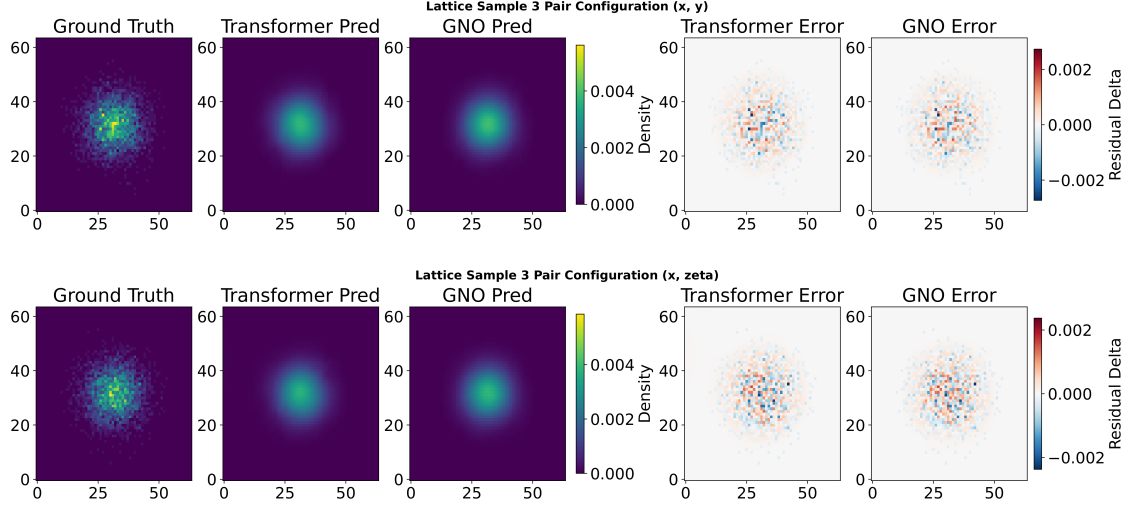
Fig. 13: Direct density-level comparison of the local-window Transformer and GNO for sample s = 3 . Top: transverse cross-plane marginal (x, y) , pair p = 0 . Bottom: mixed transverse–longitudinal marginal (x, \zeta) , pair p = 1 . Each row displays the reference density, both model predictions, and their residual fields.
