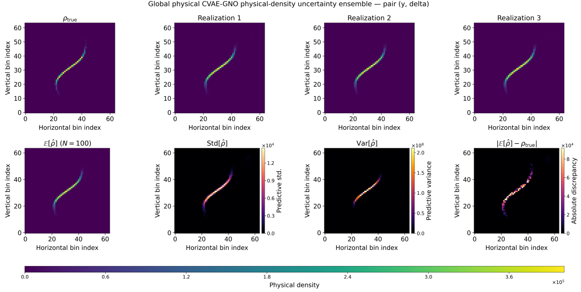
Fig. 19: Conditional latent uncertainty for the physical-density reconstruction of the same (y, \delta) marginal and validation condition. Physical bin edges are generated from the predicted centroids and RMS spread extensions. The density ensemble therefore combines uncertainty in the decoded normalized shape with variability of the physical-statistics head. The comparison is displayed in bin-index coordinates and should not be interpreted as interpolation onto a single common physical grid.
