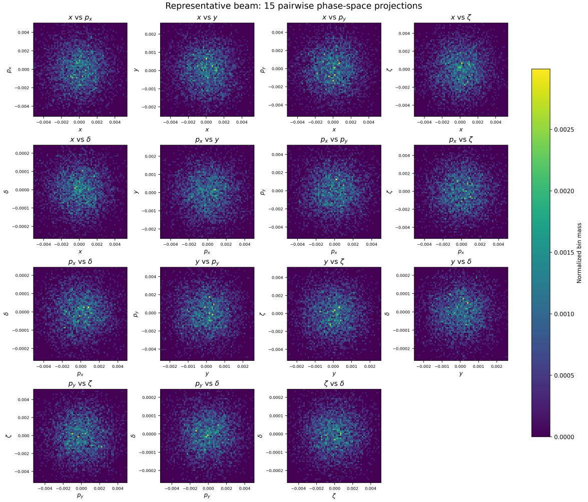
Fig. 1: Representative beam state encoded through its fifteen pairwise two-dimensional phase-space marginals. The associated centroid and coordinate-wise RMS-spread vectors retain complementary information about physical position and extension. The figure represents a reduced description of a six-dimensional state, not a unique reconstruction of the complete joint density.
