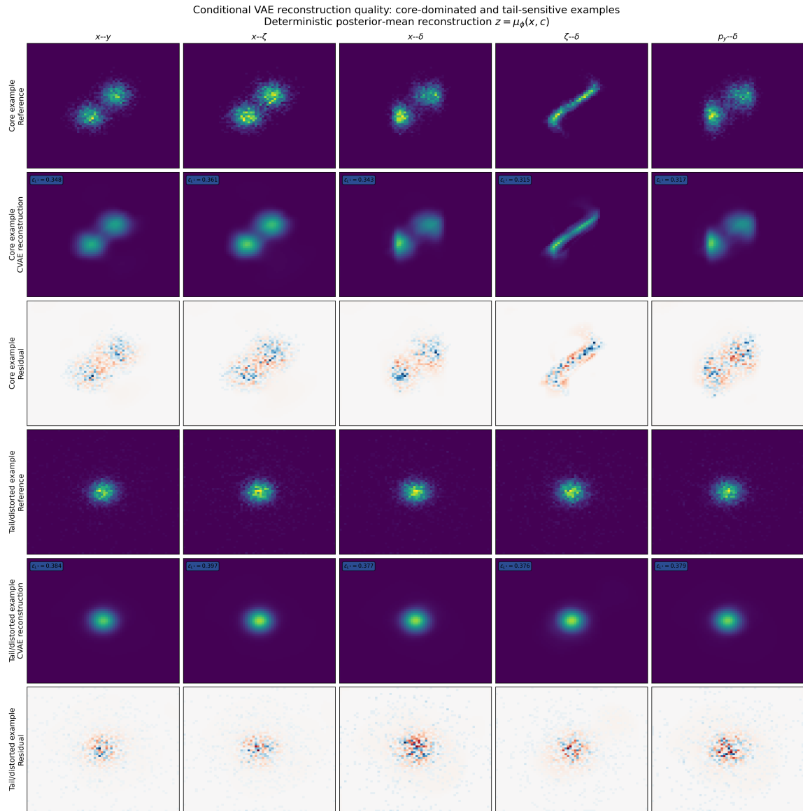
Fig. 9: Conditional VAE reconstruction quality for representative beam distributions. The comparison illustrates both the fidelity of the reconstructed high-density core and the increased difficulty associated with lower-density tails and distorted phase-space structure.
