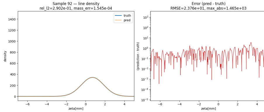
Fig. 7: Representative line density reconstruction showed along logarithmic error. The FNO prediction \hat{\lambda}_{\text{out}} is compared with the reference profile \lambda_{\text{out}} . The residual representation, \hat{\lambda}_{\text{out}} - \lambda_{\text{out}} , provides a complementary view of systematic reconstruction error.
