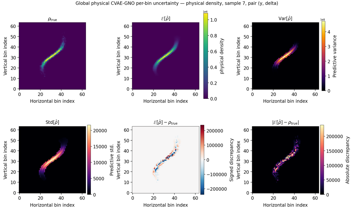
Fig. 21: Per-bin physical-density diagnostic for held-out sample s = 7 , the (y, \delta) projection, and R = 64 stochastic forward passes. The panels show the reference density, ensemble mean, predictive variance, predictive standard deviation, signed ensemble-mean discrepancy, and absolute discrepancy. The raw density scale depends on the physical coordinate units and bin area, the dimensionless discrepancy-to-spread ratios discussed in the text provide the relevant comparison between prediction error and conditional latent variability.
