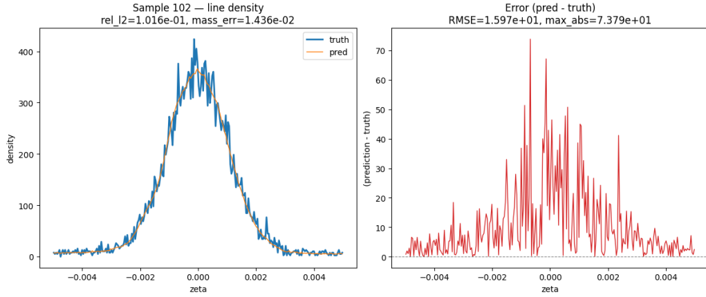
Fig. 8: Representative test-set prediction for the reduced FNO longitudinal surrogate. Randomized noise is added to the sample to illustrate the robustness of the learned operator. The figure compares the reference line density \lambda_{\text{out}} with the FNO prediction \hat{\lambda}_{\text{out}} and the residual field \hat{\lambda}_{\text{out}} - \lambda_{\text{out}} .
