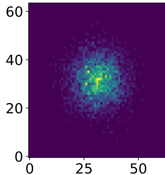
Ground Truth
