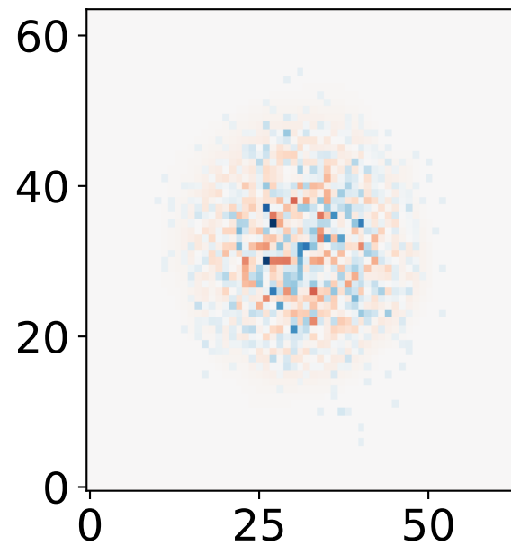
Transformer Error
