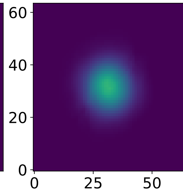
Transformer Pred
