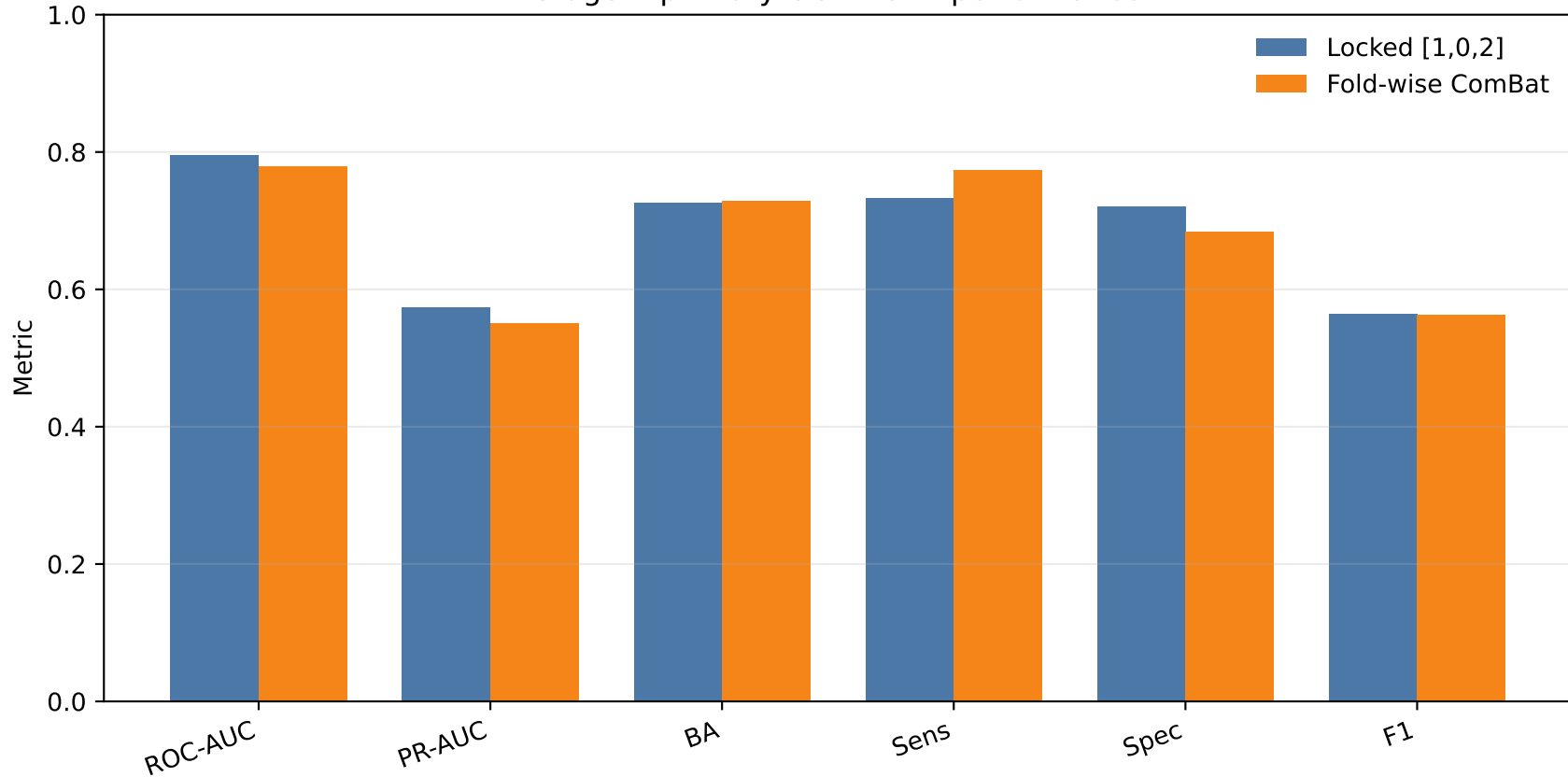
Stage-B primary OOF-ECDF performance
