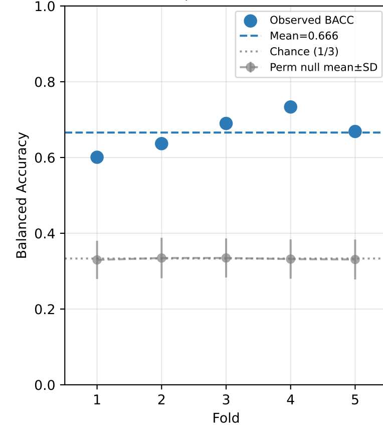
kNN-5 Manufacturer BACC vs permutation null
