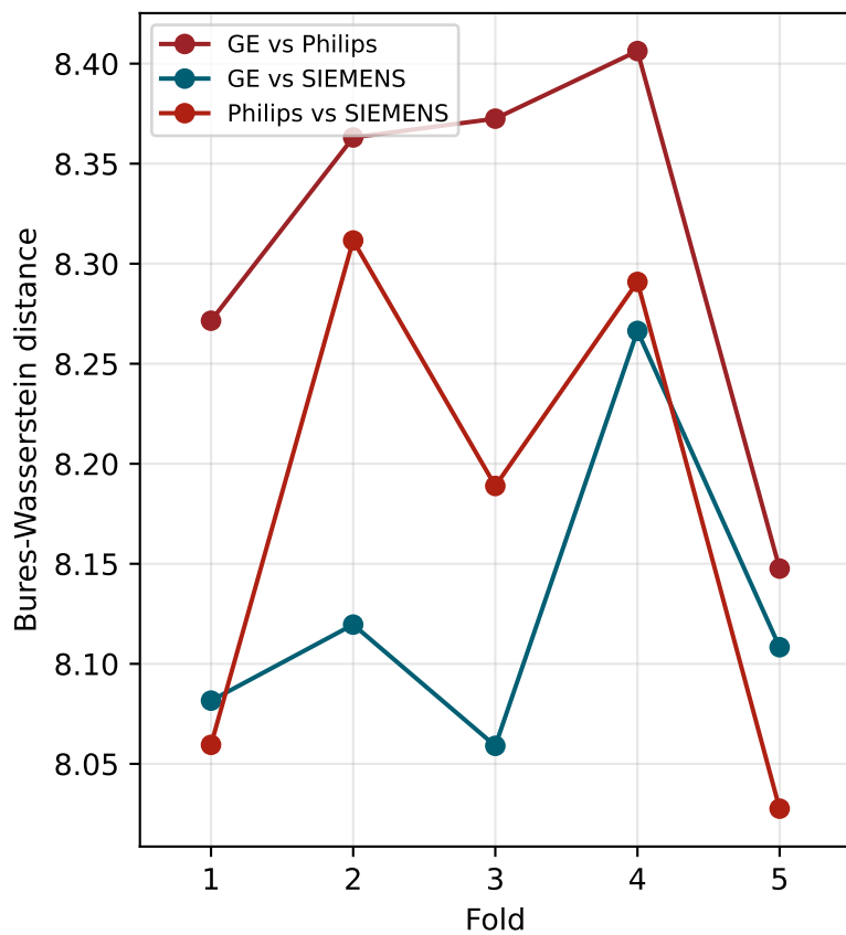
Bures-Wasserstein Distance (between manufacturer covariances)
