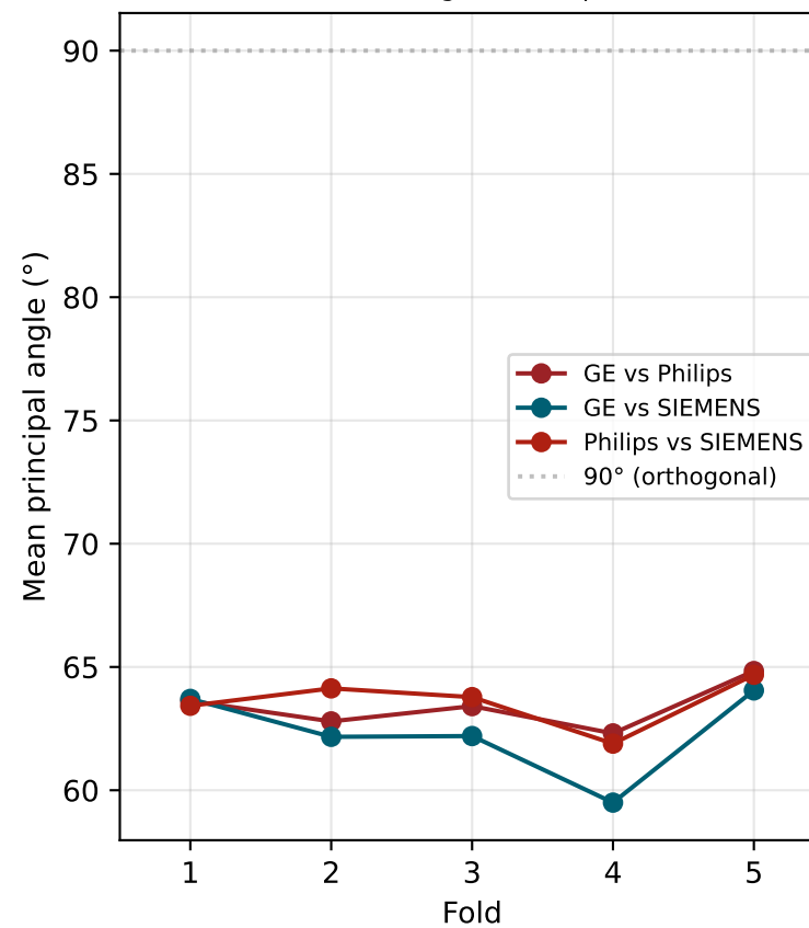
Mean Principal Angle (top-20 PCs) (90° = orthogonal subspaces)
