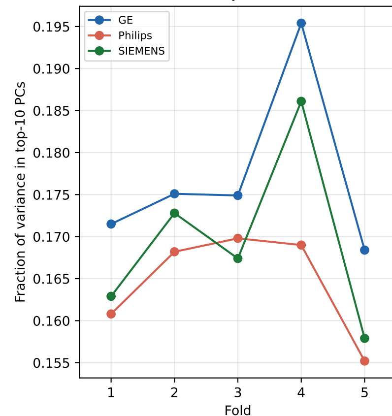
Top-10 PC Variance Fraction (dimensionality concentration)
