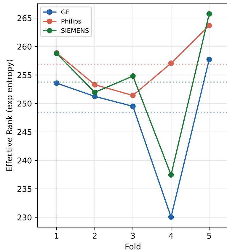
Effective Rank per Manufacturer (LW covariance, trainDev fitted)
