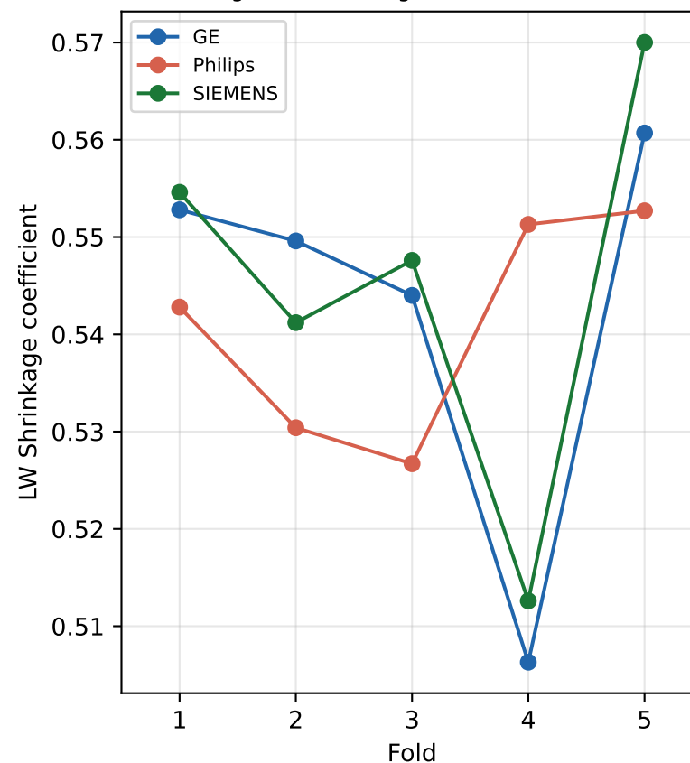
Ledoit-Wolf Shrinkage (higher = more regularization needed)
