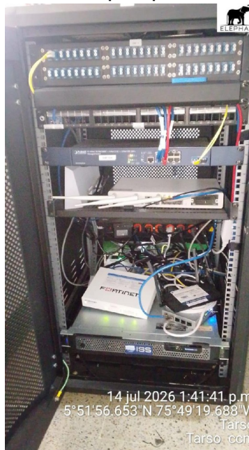
Foto patch panel
