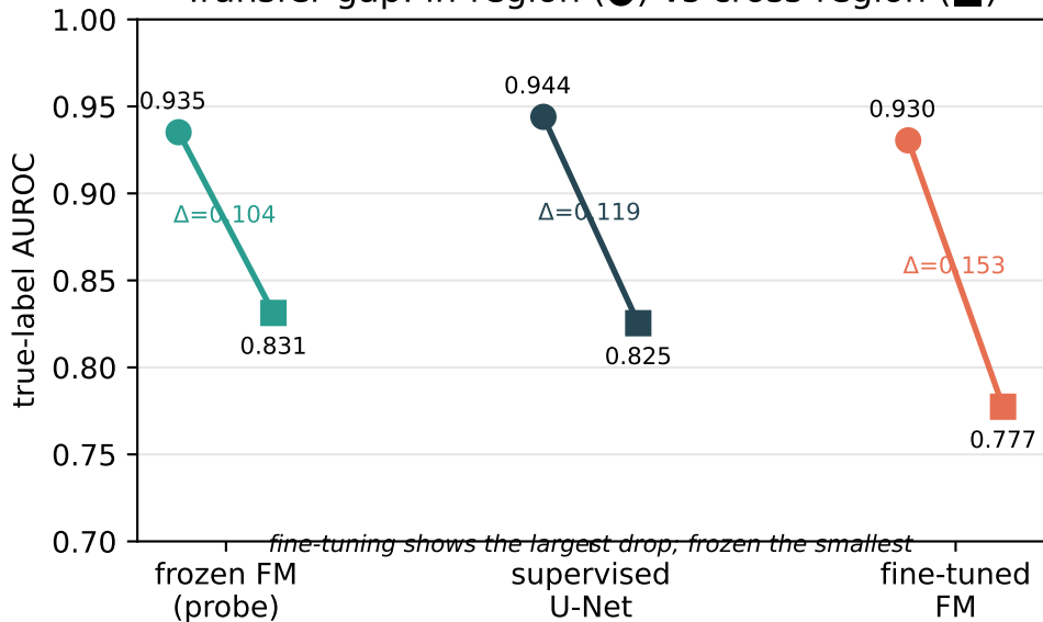
Transfer gap: in-region (●) vs cross-region (■)
