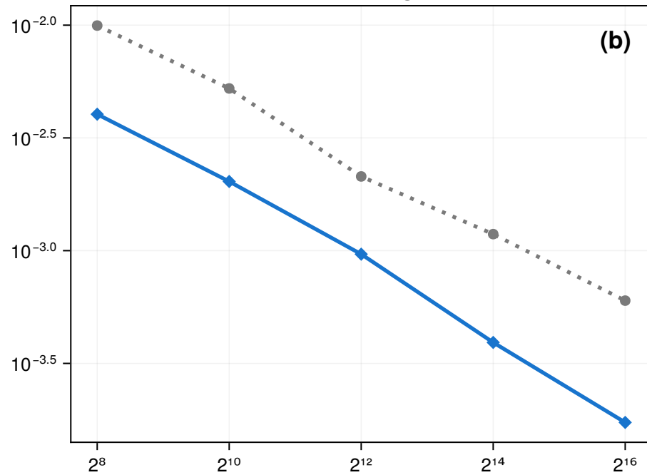
Genuine R-vine, d = 5
