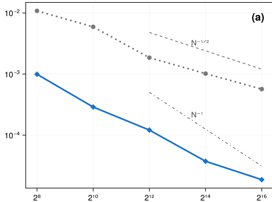
Mixed families, d = 20
