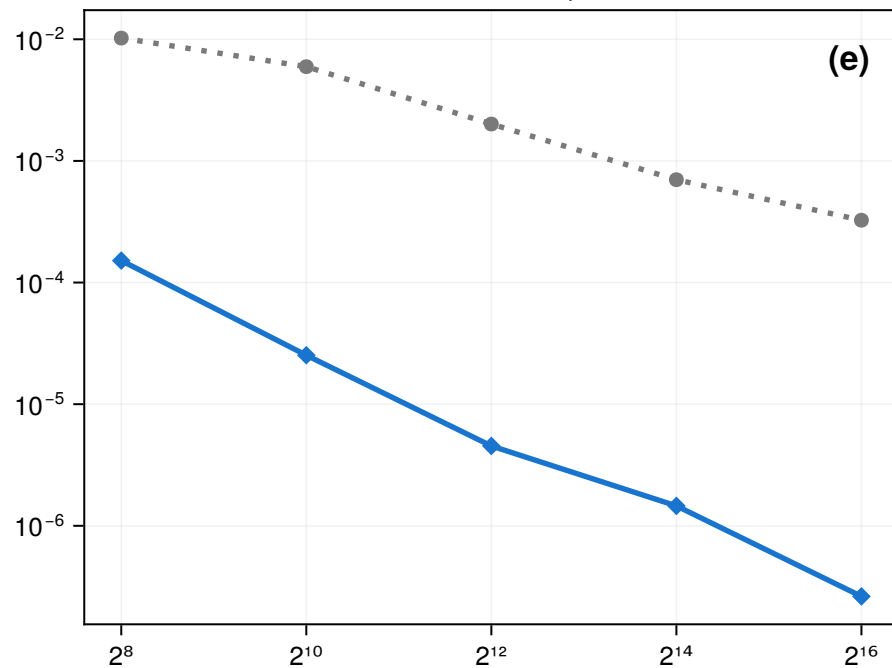
Genuine R-vine, d = 5
