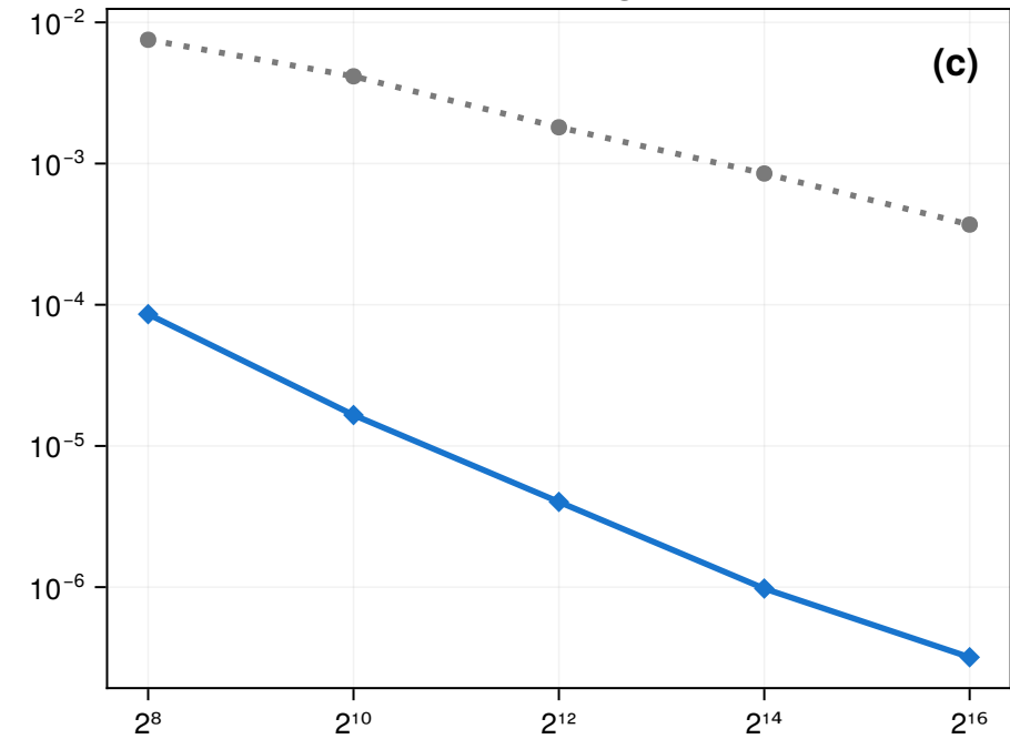
Gaussian rectangle, d = 10
