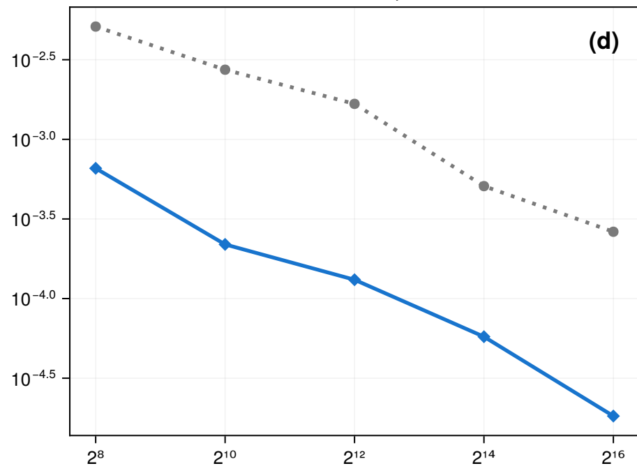
Mixed families, d = 20
