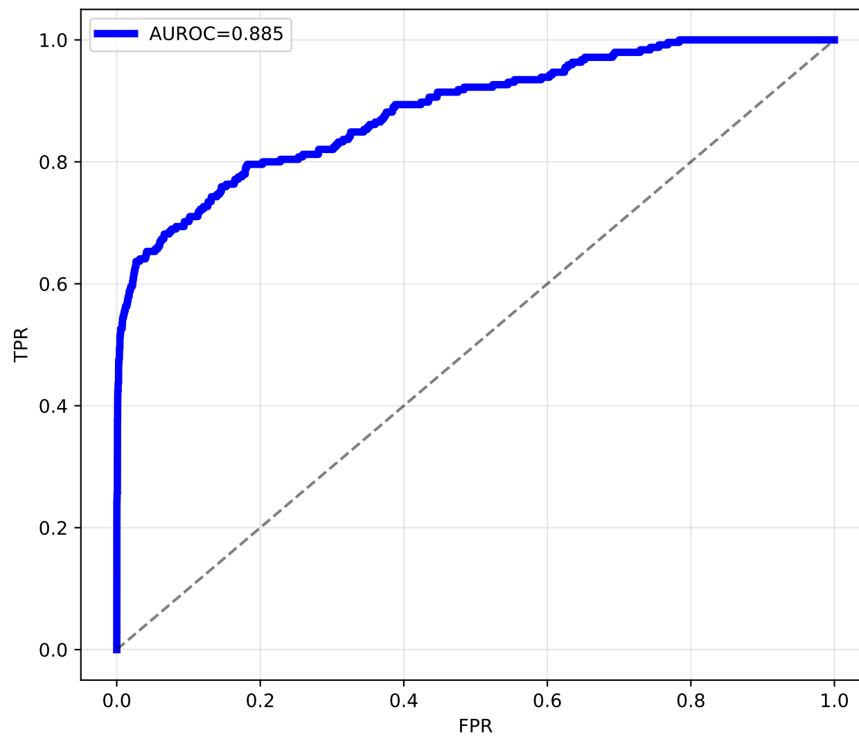
Test ROC Curve
