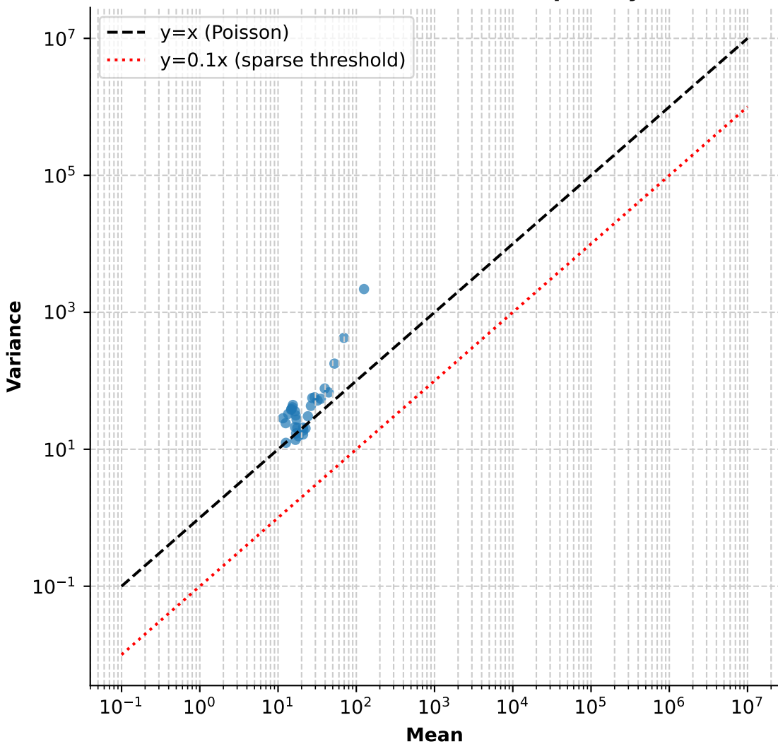
Mean vs Variance (check sparsity)
