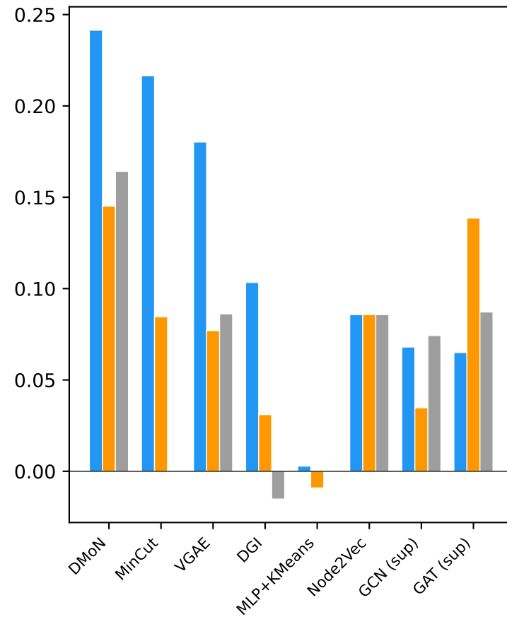
BioGRID
