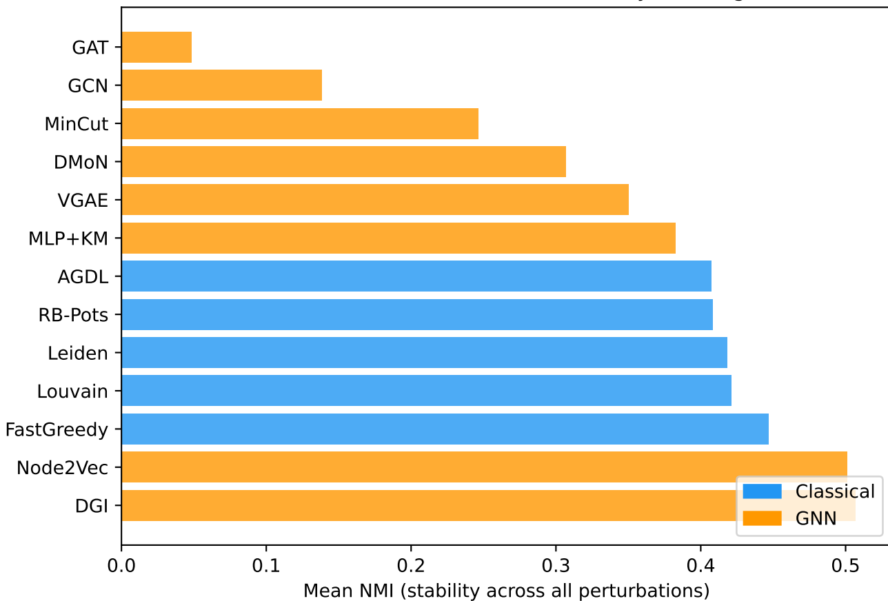
GRN: Overall Perturbation Stability Ranking
