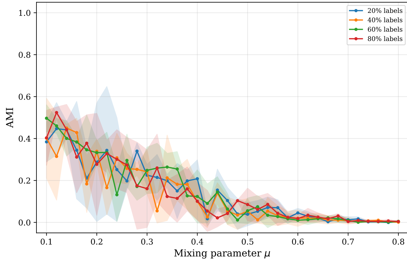
(a) GCN Label Fraction Ablation
