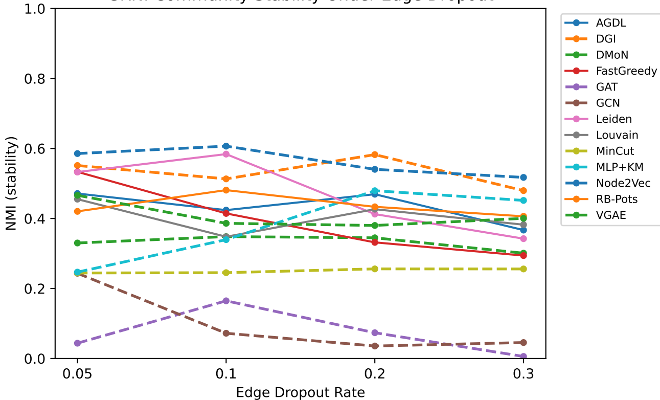
GRN: Community Stability Under Edge Dropout
