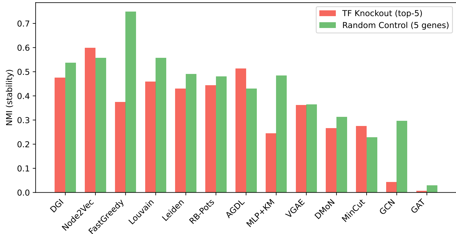
GRN: TF Knockout Impact on Community Structure
