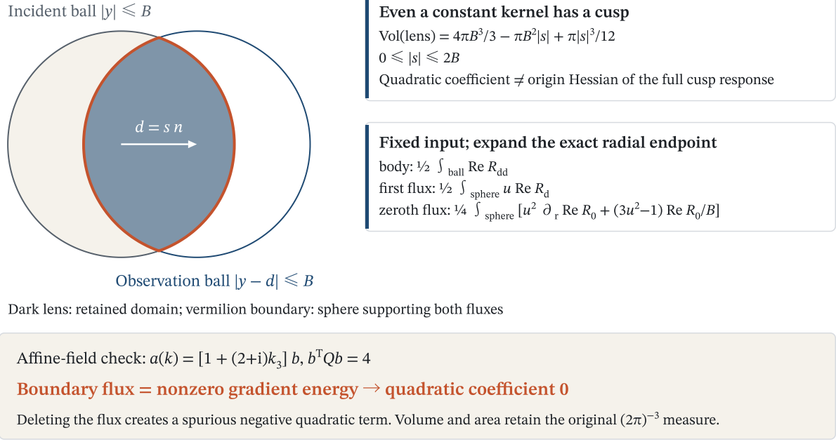
Figure 2 The sphere is not courtroom decoration. The dark region on the left is the retained two-ball intersection; its vermilion boundary marks the spherical surface supporting the two fluxes. The incoming cap outside the intersection, cut off by the observing window, produces the first-order loss corresponding to the |d| term. The right panel splits the quadratic coefficient into body, first flux and zeroth flux. The geometry is schematic; the calculation uses the exact upper limit (8.4) and original measure.
