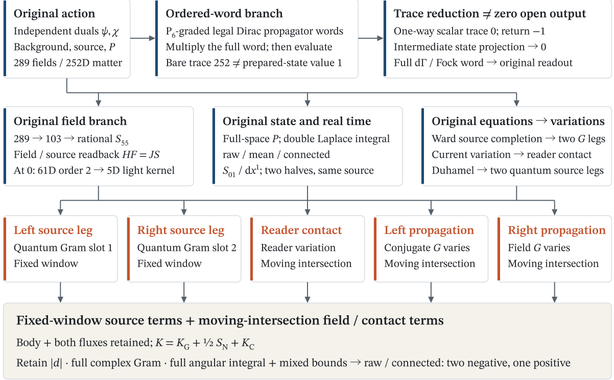
Figure 1 One original action, two testimonies; all five terms must appear. The upper branch preserves word order, grading and evaluation. The lower branch joins the original matter feedback, original-field recovery and quantum prepared-state readings. The two quantum source legs include the Duhamel variation and use fixed windows; the two propagation legs and reader contact use the two-ball intersection that moves with the external momentum. All five terms marked in vermilion are required. The window labels refer to the zero output momentum and equal-radius windows of this case; Section 7.4 gives the general window assignment. Arrows indicate dependence, not numerical equality.
