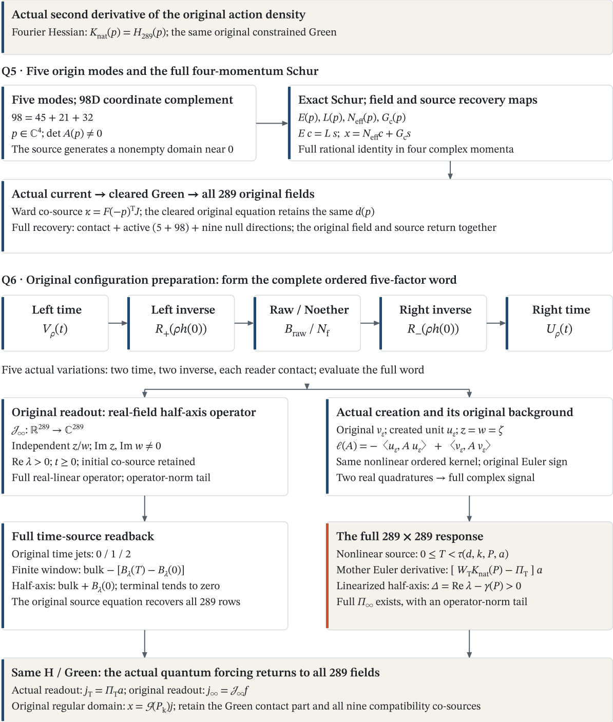
Figure 4 Original action, complete kernel and actual preparation return the same field table. The Fourier Hessian identity comes from the actual first-jet density. Q5 retains five origin directions and 45 + 21 + 32 complementary coordinates, using the complete Schur complement to recover all fields with their original denominator. Q6 applies the prepared evaluation after forming the complete word of the left and right times, both matter inverses and the original action reader; the middle contact retains the raw-to-Noether transport correction. Conditions are stated separately for the original real-field half-line, actual nonlinear finite window and complete linearized half-line: \gamma(P) = \max(0, \text{Re } P_0) , with \tau(d, k, P, a) the source-generated common window of the two actual signals. The creation-minus-background functional evaluates the complete product to generate \Pi_T ; the same two-history combination generates the time source and the two B_\lambda endpoints. The original Green matrix, contact and nine compatibility directions are retained below.
