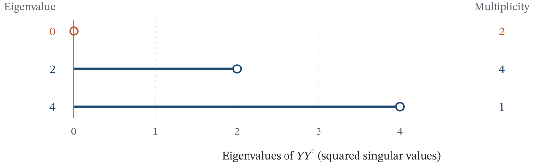
Figure A2. Nonzero singular values and kernel of the joint vacuum. The left column gives the eigenvalues of YY^\dagger (squared singular values), and the right column their multiplicities. The vermilion zero eigenvalue, of multiplicity 2, gives \text{rank } Y = 5 . The Gram matrix comes from the complete 7 \times 21 wedge map. These bare singular values have a different identity from the original frequency spectrum of §6.
