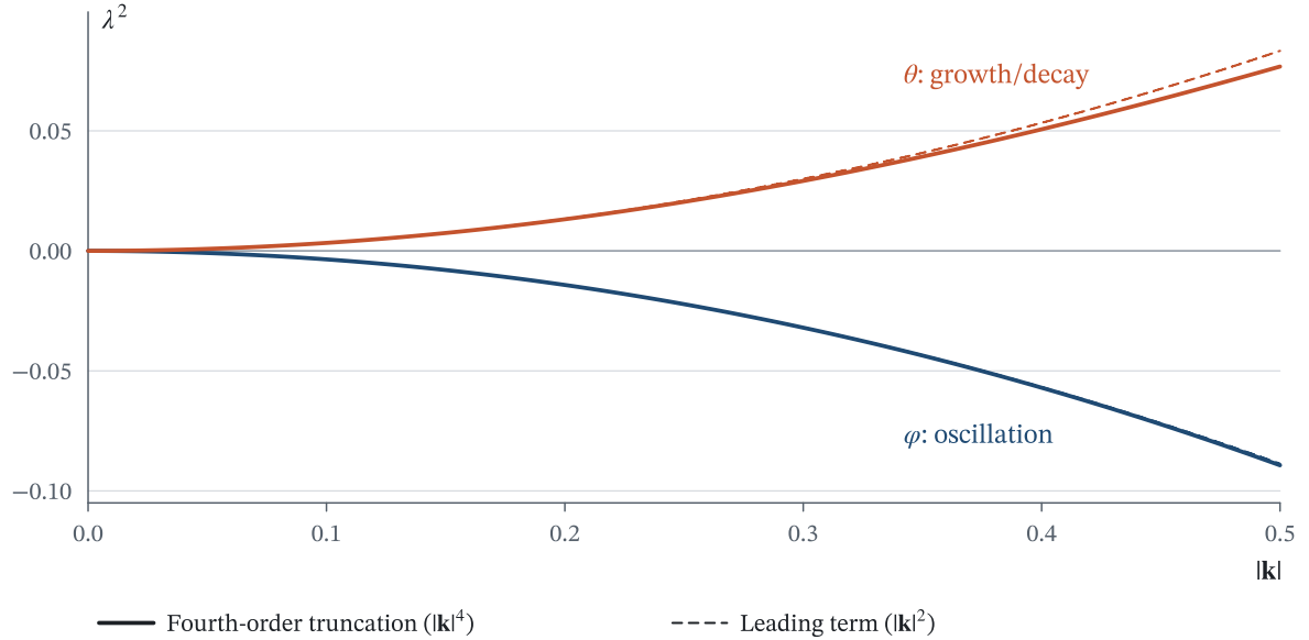
Figure 2. Two soft branches in original time. Solid curves are the fourth-order truncations in (5.10)–(5.11) near \mathbf{k} = 0 , and dashed curves are their second-order leading terms. The horizontal axis shows 0 \leq |\mathbf{k}| \leq 0.5 ; the asymptotic remainder is O(|\mathbf{k}|^6) . The vertical axis is the original-time growth variable \lambda^2 . Below zero lies the oscillatory \varphi branch (deep blue); above zero lies the growth/decay \theta branch (vermilion), whose fourth-order term visibly separates it from its leading term over the displayed range. These truncations are not exact finite-momentum dispersion relations.
