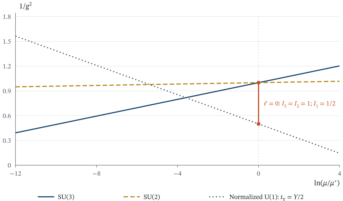
Figure A1. Three affine readings for the specified inventory. The horizontal axis is the inventory running coordinate \ln(\mu/\mu^*) , distinct from original time. With \ell = \ln(\mu/\mu^*)/(8\pi^2) , the three lines are (A.2), using native \sigma = 1/2 with no thresholds, experimental fit, or GeV calibration. The vermilion vertical segment marks the gap at \ell = 0 : I_3 = I_2 = 1 , while I_1 = 1/2 .
