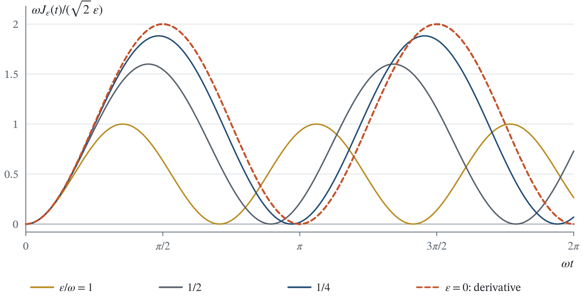
Figure 3. How the finite current approaches its actual derivative. The solid curves use (8.14) with \epsilon/\omega = 1, 1/2, 1/4 (gold, gray, and dark blue). The vermilion dashed curve is the normalized derivative 1 - \cos 2\omega t , with \omega = 18\sqrt{15}/125 . The horizontal coordinate \omega t uses original time, not proper time. The vertical coordinate is \omega J_\epsilon/(s\epsilon) for a unit occupied state; the current of the field with its original amplitude is four times as large. Finite amplitude changes both amplitude and oscillation frequency.
