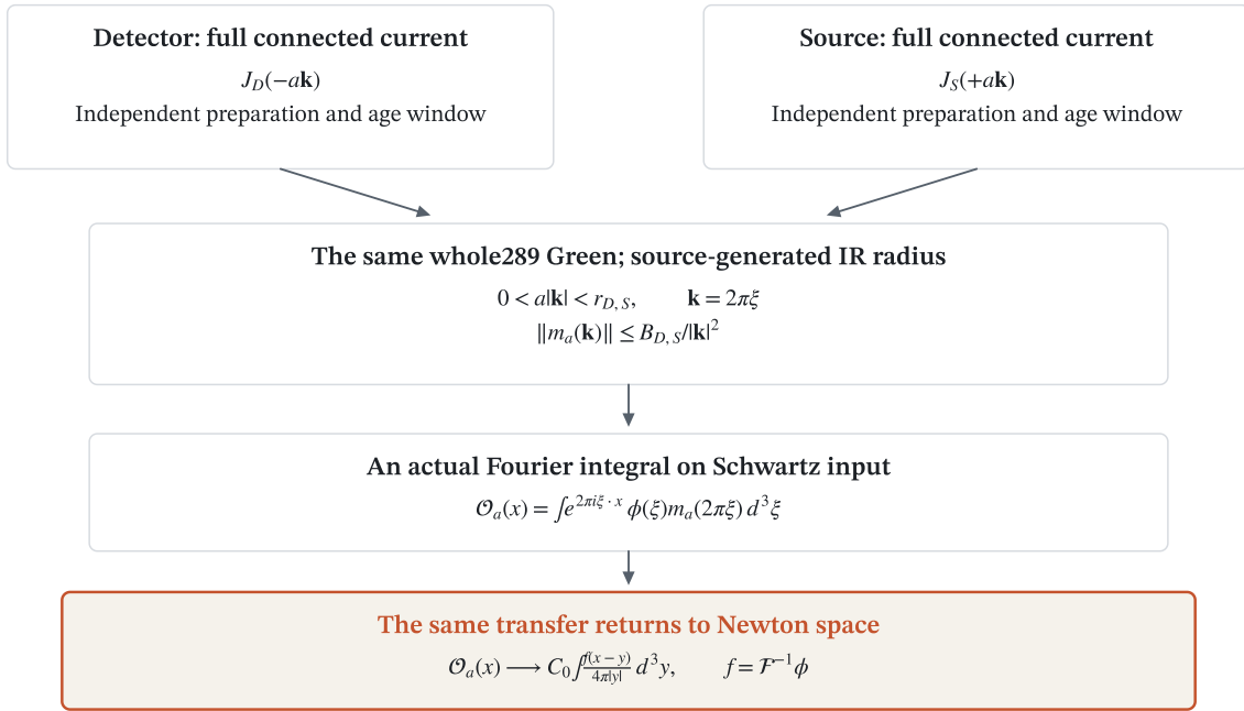
Figure 5. Two actual endpoints share one Fourier transfer. The created N2 connected currents use J_D(-a\mathbf{k}) and J_S(a\mathbf{k}) with independent preparations and age windows. Here m_a is the complete endpoint contraction in (12.11), and C_0 = L(0, S_0) . Actual continuity and the all-direction Green function generate the common infrared radius and budget; the symbol is zero outside its defined window. Schwartz input pays for the same genuine integral, with f = \mathcal{F}^{-1}\phi and exactly one 4\pi . This raw connected readout keeps the normalization in (12.9), with no additional hc_b divisor.
