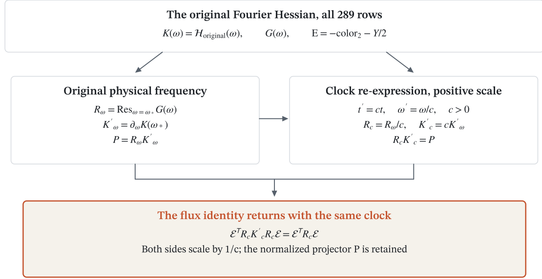
Figure 4. Clock re-expression of the same original action. Fix an original source branch, a unit spatial direction, and the generated simple-pole range. A positive clock change t' = ct gives R_c = R_\omega/c and K'_c = cK'_\omega . Here \mathcal{E} inserts the literal E into four gauge slots on all 289 directions: mixed outputs are retained before contraction. The normalized projector and flux identity are preserved while both tensors scale by 1/c , as in (11.9)–(11.11).
