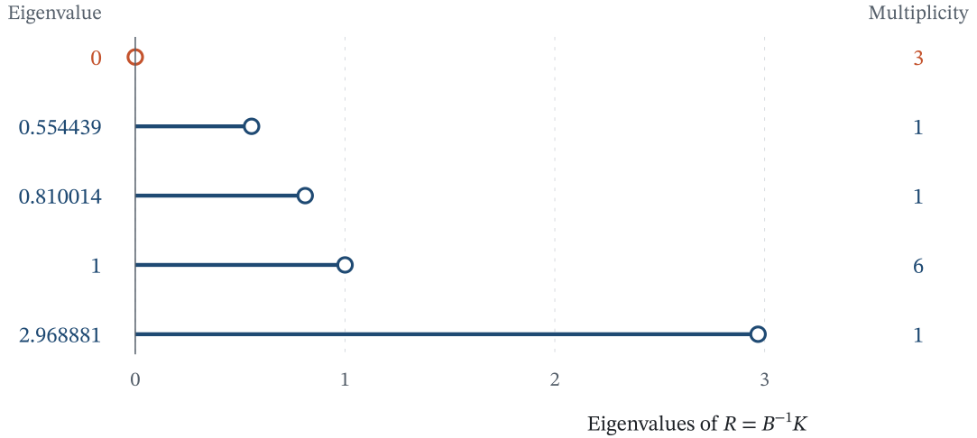
Figure A3. The native P286 bare scalar–gauge quadratic block. The left column gives the eigenvalues of R = B^{-1}K , with B the native real scalar pairing; the right column gives multiplicities. Of the 12 directions, 3 are zero (vermilion) and 9 are positive. The three nonrational eigenvalues are the roots of the cubic in (A.5), shown as decimals from rational isolating intervals. The kernel corresponds to the stabilizer tangent space; complete coupled propagation is treated separately in §4.
