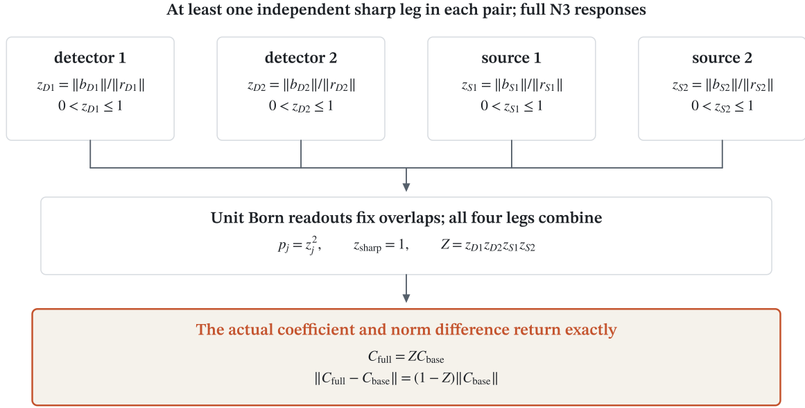
Figure 6. Four Born overlaps generate the actual Coulomb dressing. D1/D2 are the detector left/right legs; S1/S2 are the source left/right legs. Each b_j is the original bottom response, r_j the full N3 response, and p_j = z_j^2 the unit-state (3, 0) Born value. At least one leg in each pair is independently sharp; this returns the complete gauge numerator to the bottom grade while retaining both full norms. Their four positive overlaps give the coefficient and norm difference in (13.8), and enter the same whole289 Newton packet.
