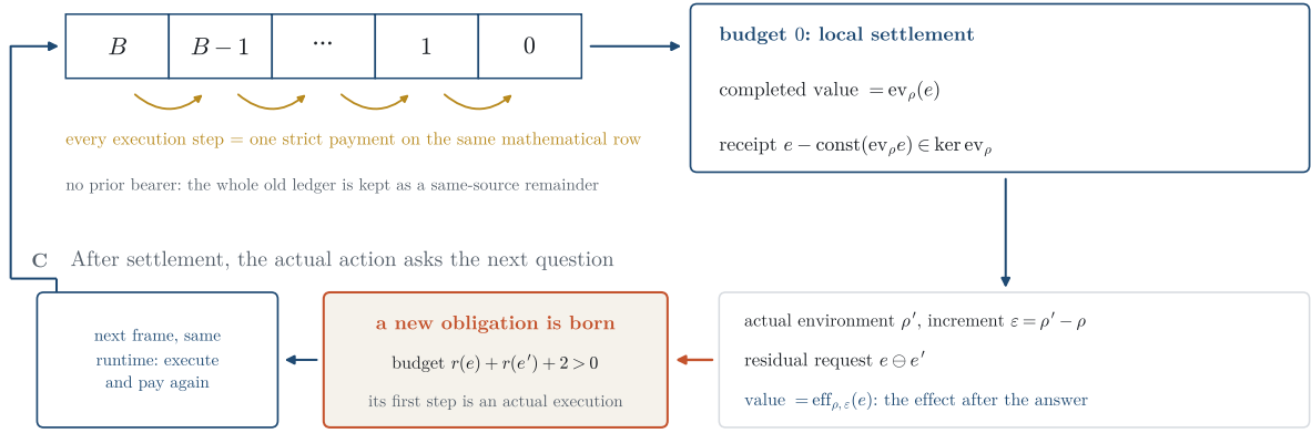
Example 8.13: x answers 1 at x \mapsto 1 ; the environment moves to x \mapsto 0 , the next question has value -1 and budget 3
