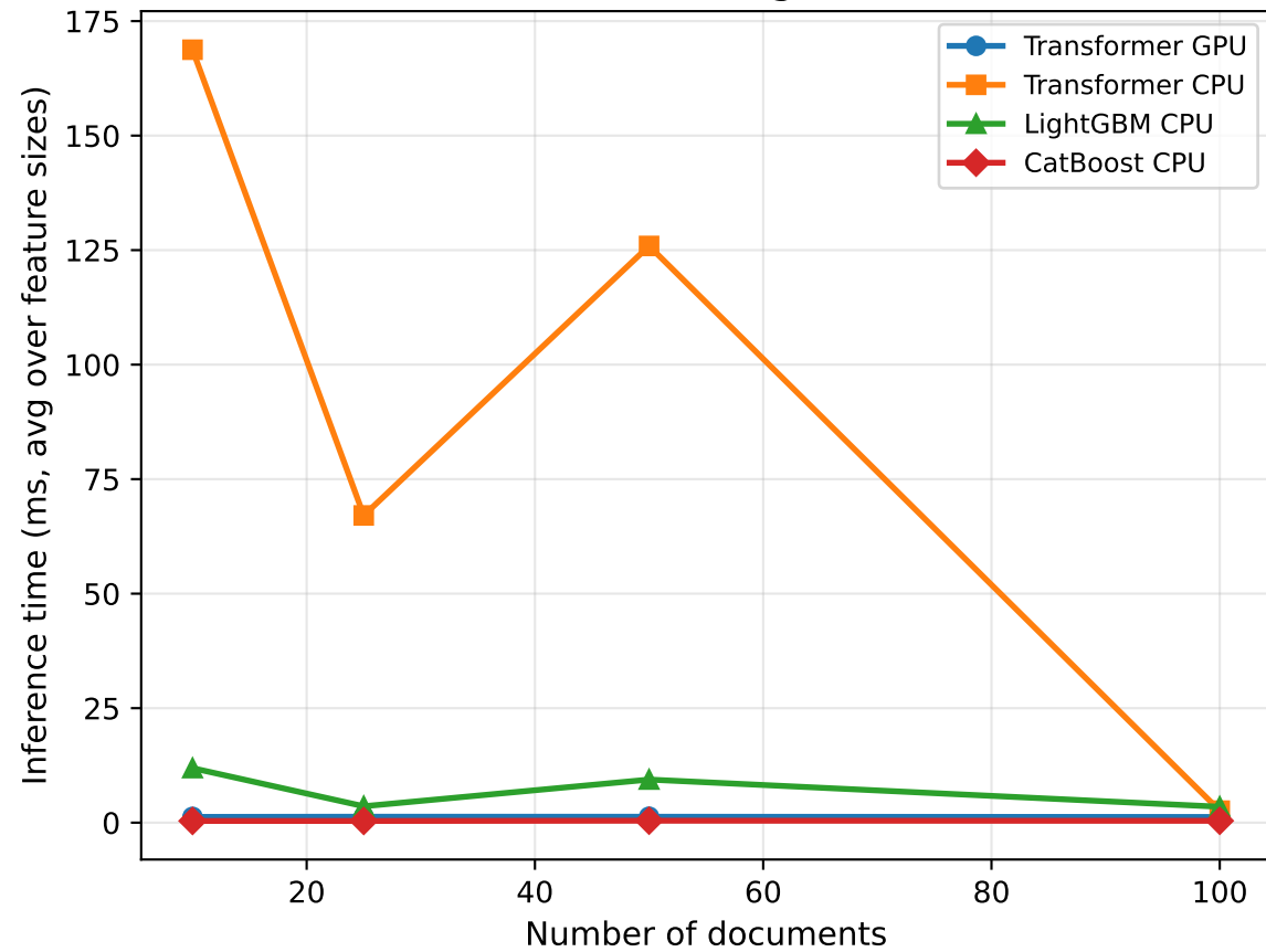
Transformer GPU/CPU vs LightGBM vs CatBoost
