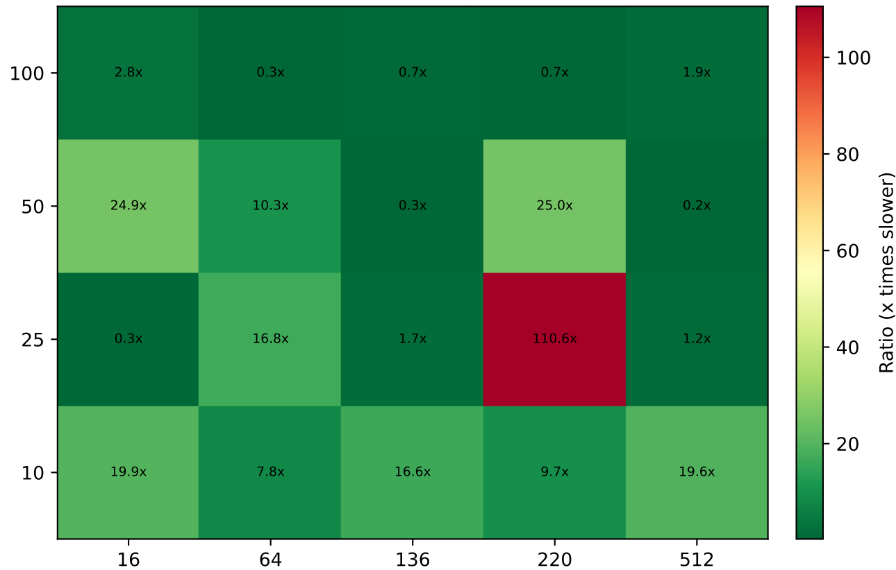
Transformer GPU/CPU vs LightGBM vs CatBoost
