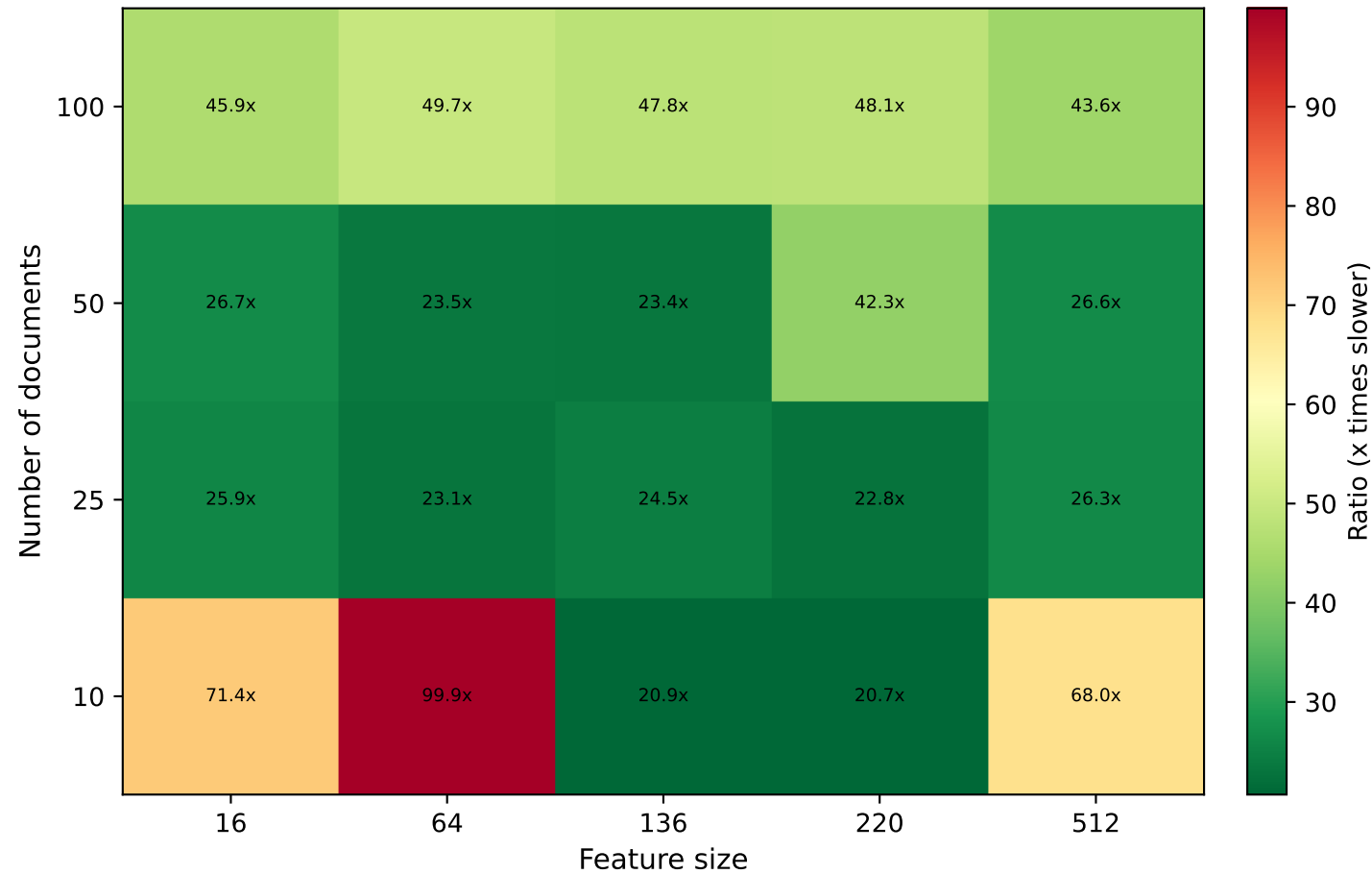
CPU: Transformer/LightGBM Speed Ratio
