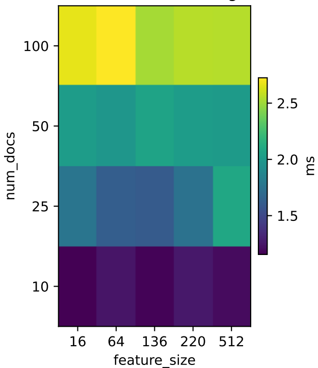
Transformer CPU wall avg (ms)
