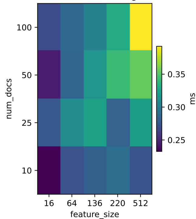
CatBoost CPU wall avg (ms)
