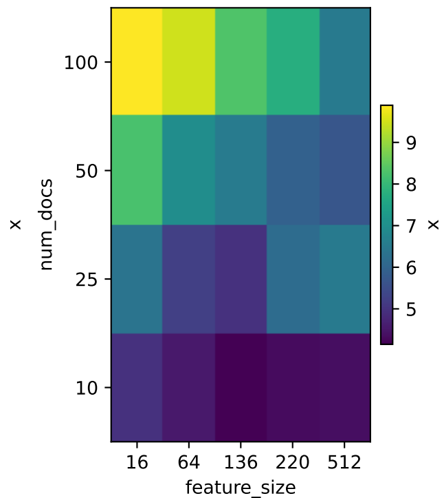
Transformer/CatBoost CPU ratio
