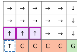
Learned robust
