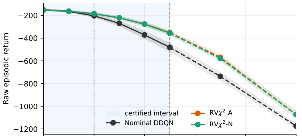
Frozen reporting robustness profile (10 training seeds)
