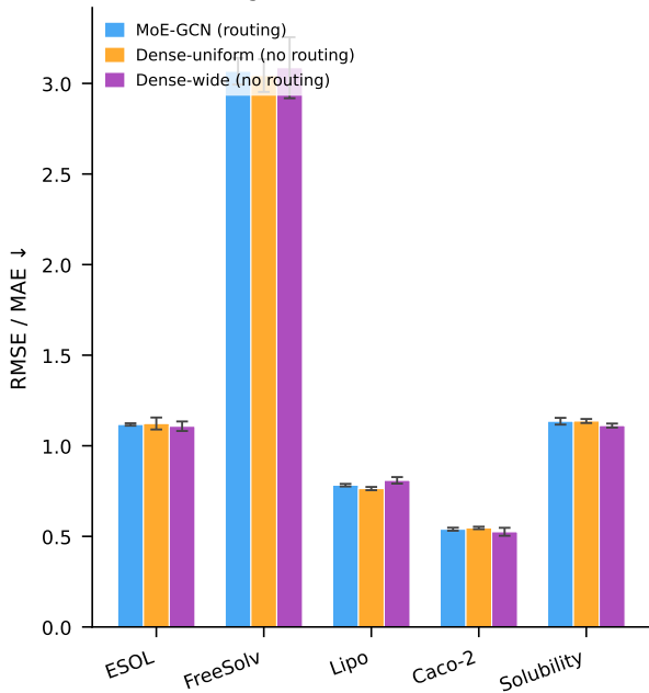
A Ablation: routing vs no routing (5 regression datasets, 5 seeds)
