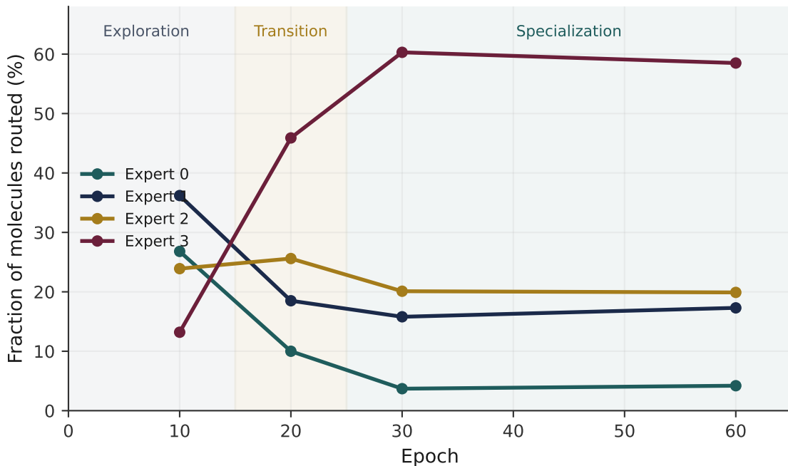
Fig. 2 | Training-time phase transition in expert routing (Tox21, 4 experts, top-1 routing)
