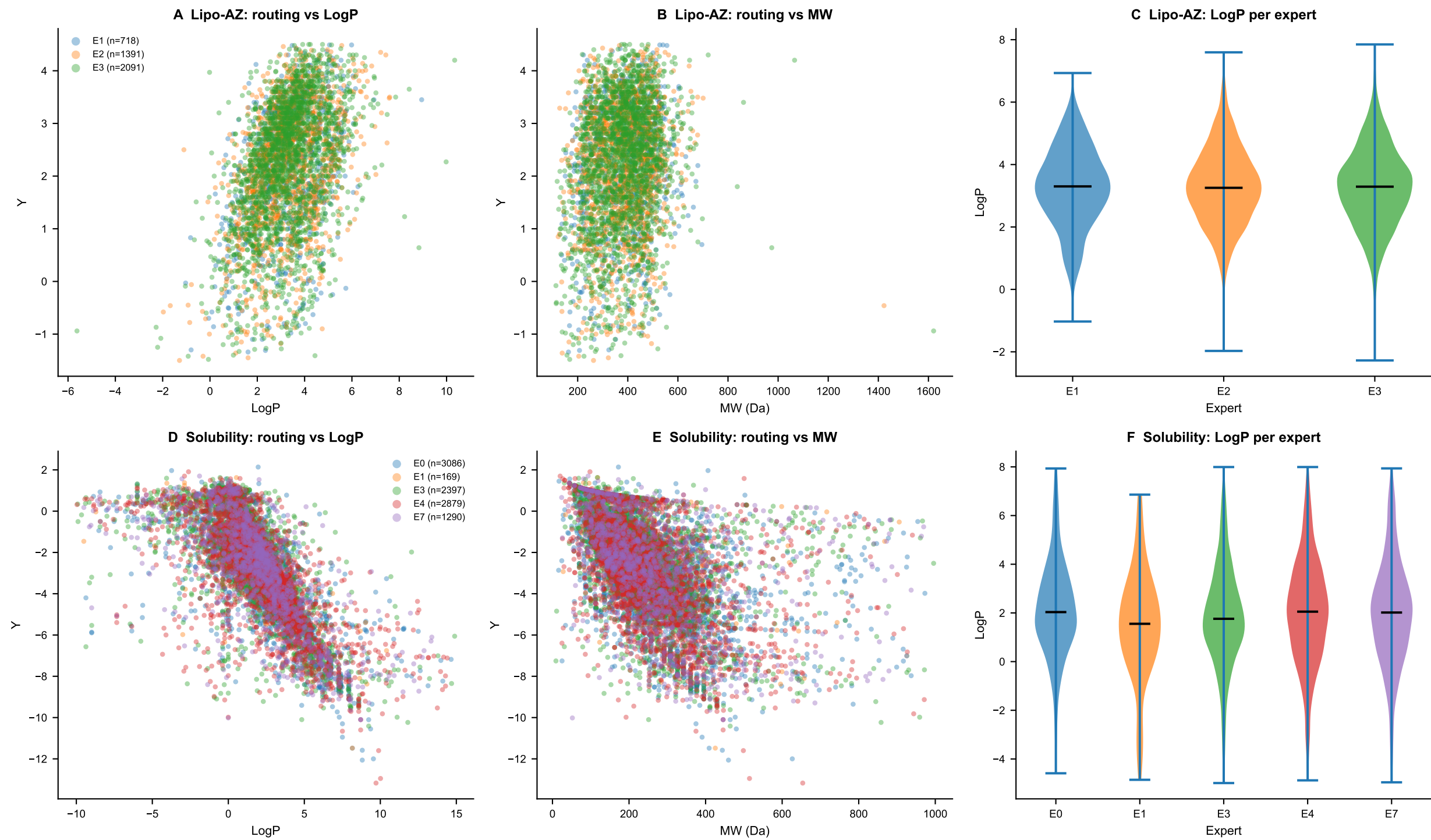
Figure 3 | Expert routing partitions chemical space (seed 1)
