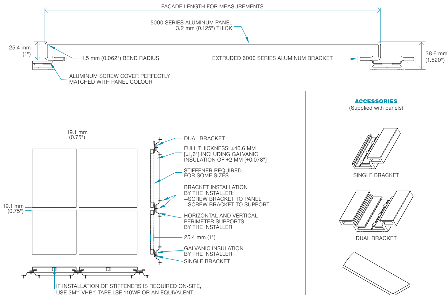
BOTH 25.4 mm (1") AND 31.75 mm (1.25") SCREW COVERS
