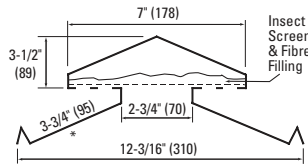
1170 VENTED ENDWALL
