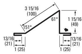
#80 2" SNOW CONTROL
