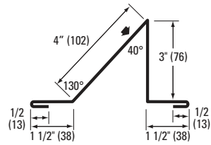
#85 3" SNOW CONTROL
