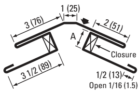
#100 RIDGE COVER
