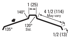
#100 RIDGE COVER
