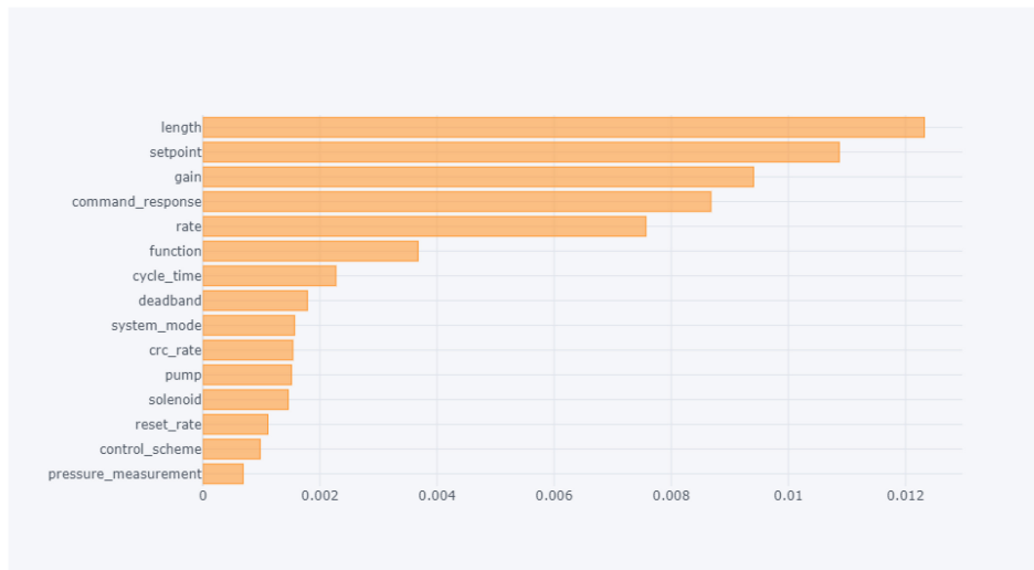
Fig. 6. Global explanation of detection framework. It displays feature ranking ordered from uppermost to lowermost. The magnitude of ranking is shown in the x axis.
