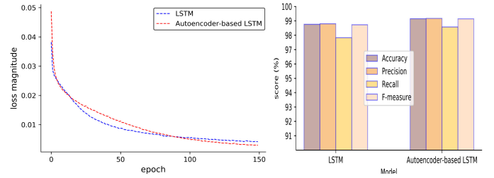
Fig. 4. Comparison of autoencoder-based LSTM and simple LSTM for loss and evaluation metrics.
