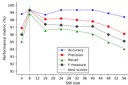
Fig. 7. Performance comparison of proposed framework using different S values of SW.
