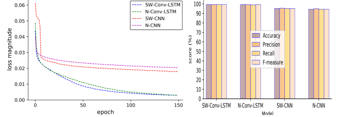
Fig. 3. Comparison of loss and evaluation metrics after the effect of two-step SW.
