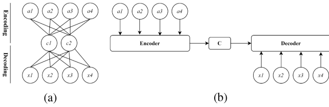
Fig. 1. Autoencoders' architecture. (a) represents the typical autoencoder architecture applied using fully connected neurons while (b) denotes the autoencoder based on RNN architecture which is effective for dealing with sequential information.
