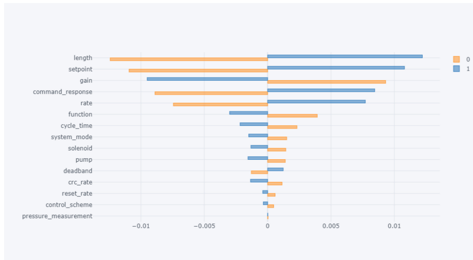
Fig. 5. Inference graph across the two classes. This visualization shows which feature was more vital in predicting a specific class.
