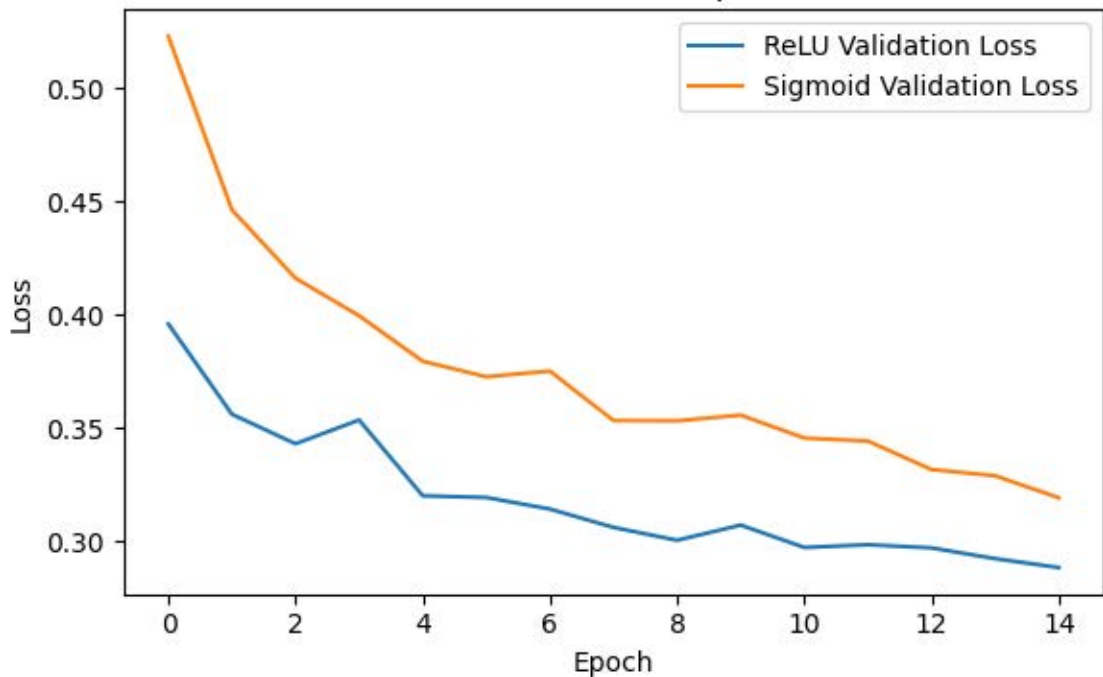
Validation Loss Comparison
