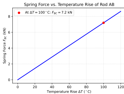
Fig. 4.5. Force in spring BC versus temperature rise of rod AB
