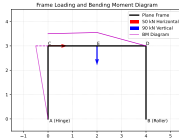
Fig. 4.1. Frame loading and bending moment diagram
