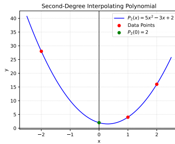
Fig. 4.3. Interpolating polynomial through the given points
