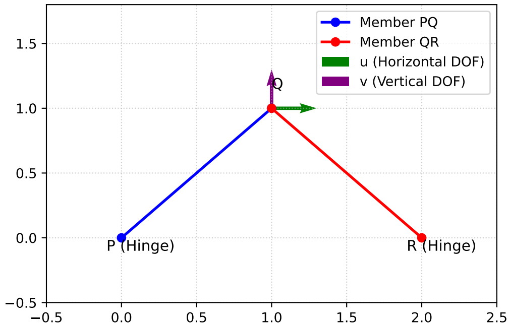
Two-Member Truss with Degrees of Freedom ( u , v ) at Q
