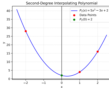
Fig. 1.1.17.1. Interpolating polynomial through the given points
