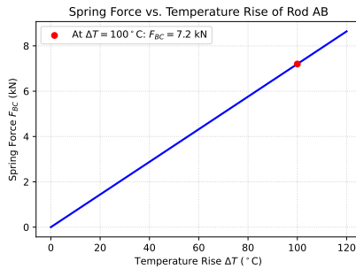
Fig. 1.1.19.1. Force in spring BC versus temperature rise of rod AB
