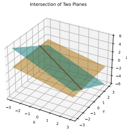
Fig. 1.1.6.1. The two planes and their line of intersection
