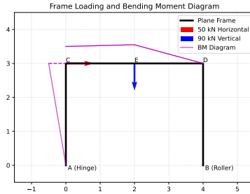
Fig. 1.1.15.1. Frame loading and bending moment diagram
