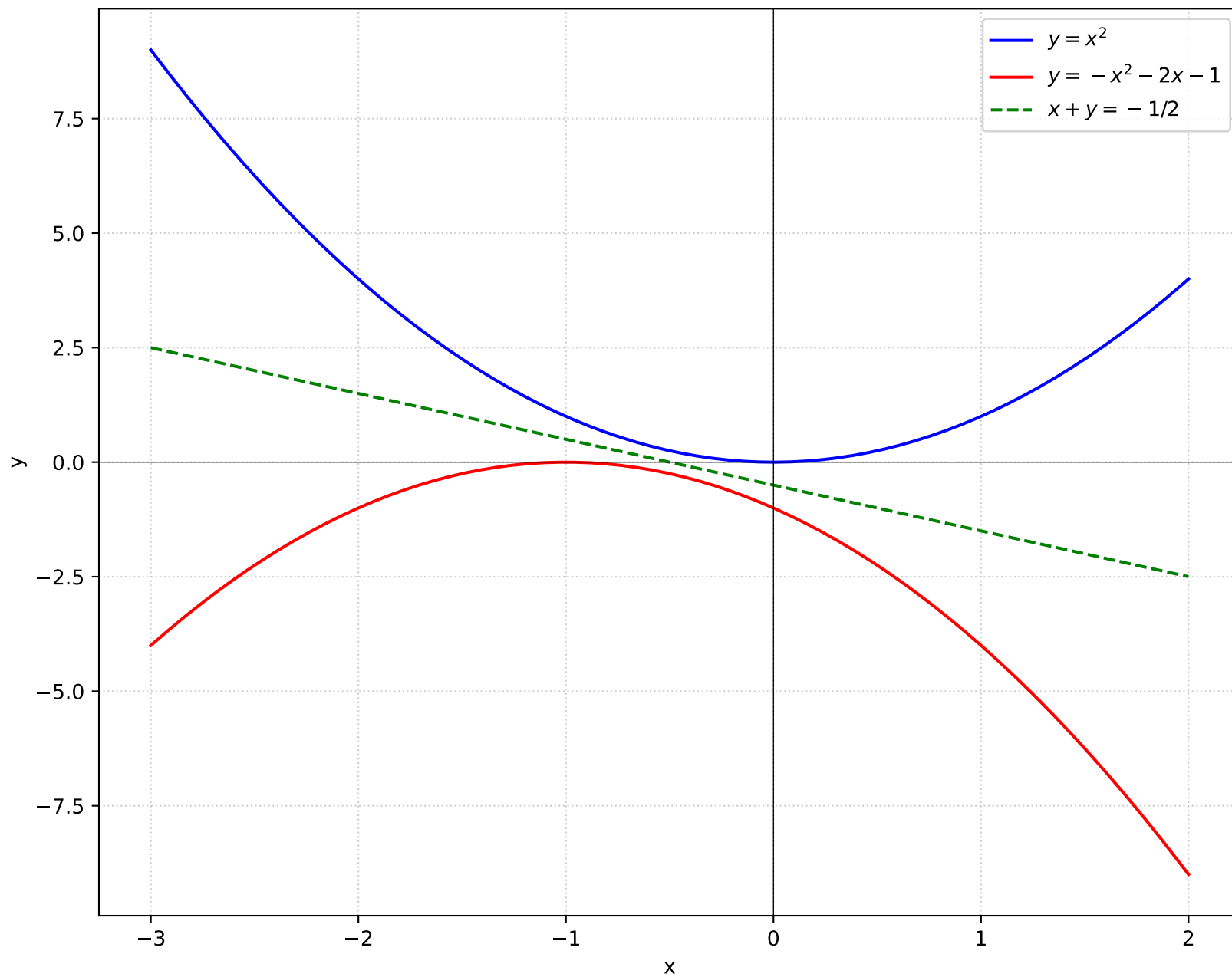
Two Parabolas and Common Line
