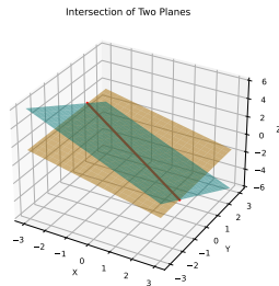
Fig. 1.2.0.4. The two planes and their line of intersection
