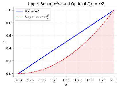
Fig. 1.2.0.5. The integrand attains its upper bound \frac{x^2}{4} only for f(x) = \frac{x}{2}
