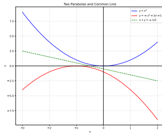
Fig. 1.2.0.1. The two parabolas and the line x + y = -\frac{1}{2} from the pencil
