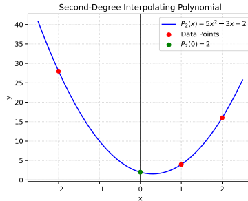
Fig. 1.2.0.9. Interpolating polynomial through the given points
