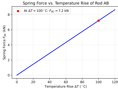
Fig. 1.2.0.11. Force in spring BC versus temperature rise of rod AB
