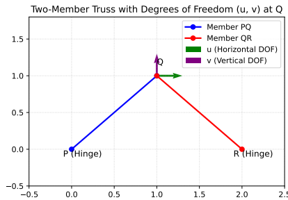
Fig. 1.2.0.6. Two-member truss with degrees of freedom u, v at Q
