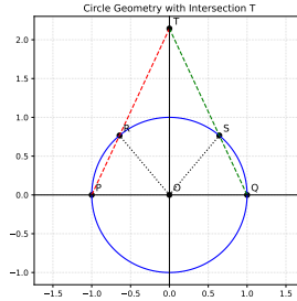
Fig. 1.2.0.2. Circle with diameter PQ , \angle ROS = 80^\circ and \angle RTS = 50^\circ
