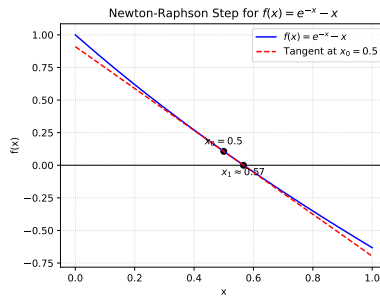
Fig. 1.2.0.8. One Newton-Raphson step for f(x) = e^{-x} - x from x_0 = 0.5
