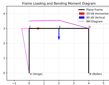
Fig. 1.2.0.7. Frame loading and bending moment diagram
