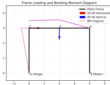
Fig. 1.2.0.7. Frame loading and bending moment diagram
