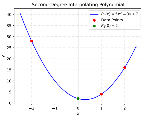
Fig. 1.1.16.1. Interpolating polynomial through the given points
