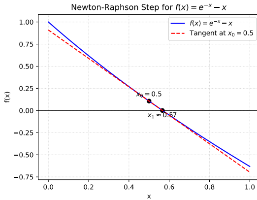
Fig. 1.1.15.1. One Newton-Raphson step for f(x) = e^{-x} - x from x_0 = 0.5
