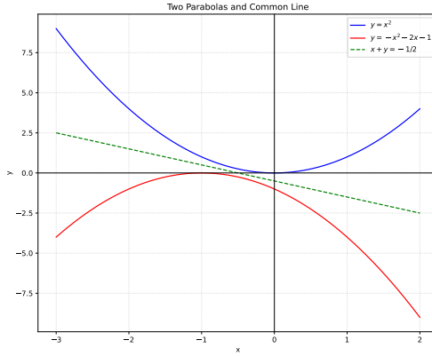
Fig. 1.1.1.1. The parabolas y = x^2 and y = -x^2 - 2x - 1
