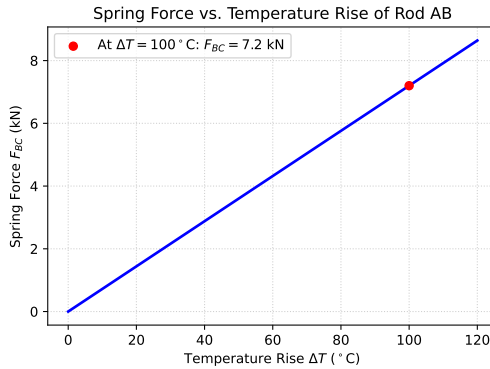
Fig. 1.1.18.1. Rod AB connected in series with spring BC under thermal loading
