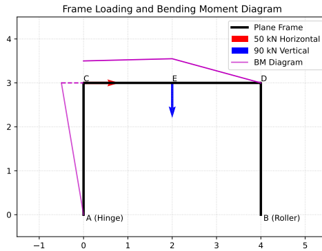
Fig. 1.1.14.1. Frame loading and bending moment diagram
