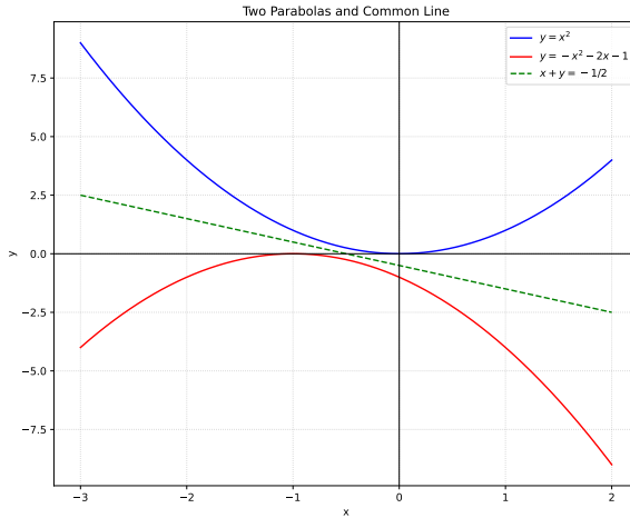
Fig. 6.1. The parabolas y = x^2 and y = -x^2 - 2x - 1
