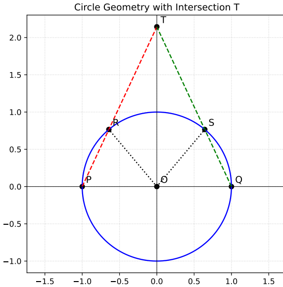
Fig. 4.1. Circle with diameter PQ , \angle ROS = 80^\circ and \angle RTS = 50^\circ
